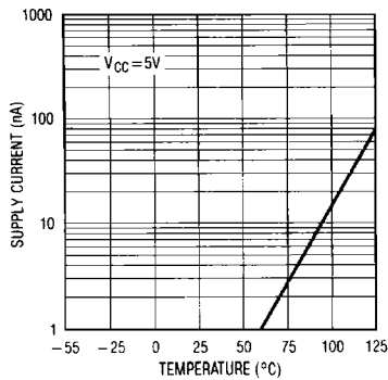
Supply Current in Shutdown
