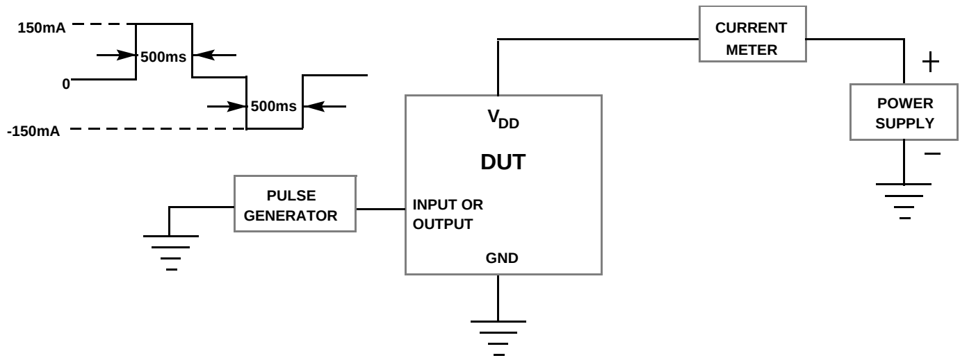
Figure 43. Latchup Test
