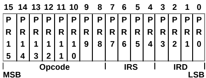
Figure 22. Program Register (PR)
