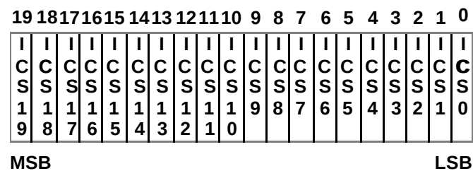
Figure 20. RISC Instruction Counter Save Register (ICS)
