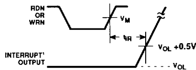
Figure 3. Port Timing
