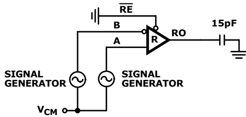
FIGURE 5A. TEST CIRCUIT
