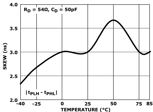
FIGURE 16. DRIVER DIFFERENTIAL SKEW vs TEMPERATURE (ISL31493E, ISL31495E)
