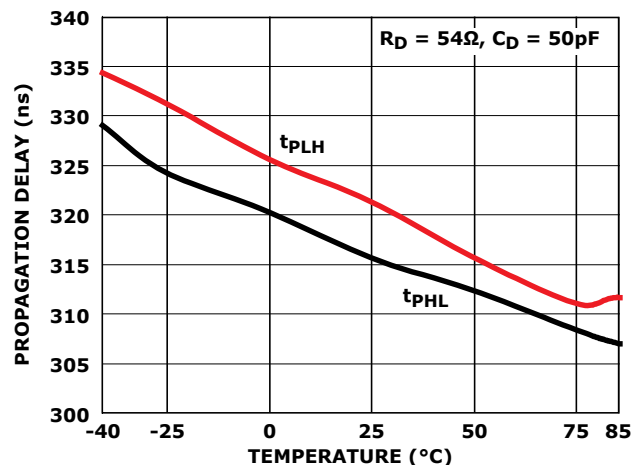
FIGURE 13. DRIVER DIFFERENTIAL PROPAGATION DELAY vs TEMPERATURE (ISL31490E, ISL31491E, ISL31492E)
