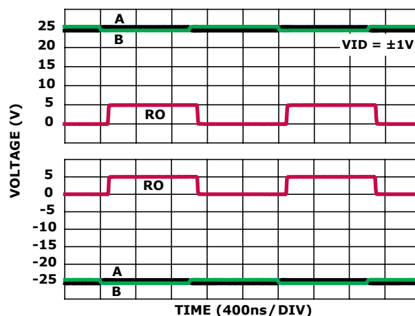
FIGURE 20. \pm 25V RECEIVER PERFORMANCE (ISL31493E, ISL31495E)
