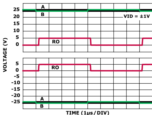
FIGURE 19. \pm 25V RECEIVER PERFORMANCE (ISL31490E, ISL31491E, ISL31492E)
