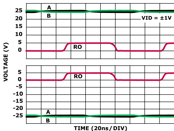
FIGURE 21. \pm 25V RECEIVER PERFORMANCE (ISL31496E, ISL31498E)
