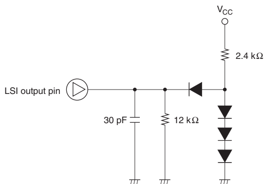
Figure 22.7 Output Load Circuit
