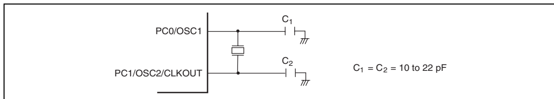
Figure 5.12 Example of Connection to Crystal Resonator
