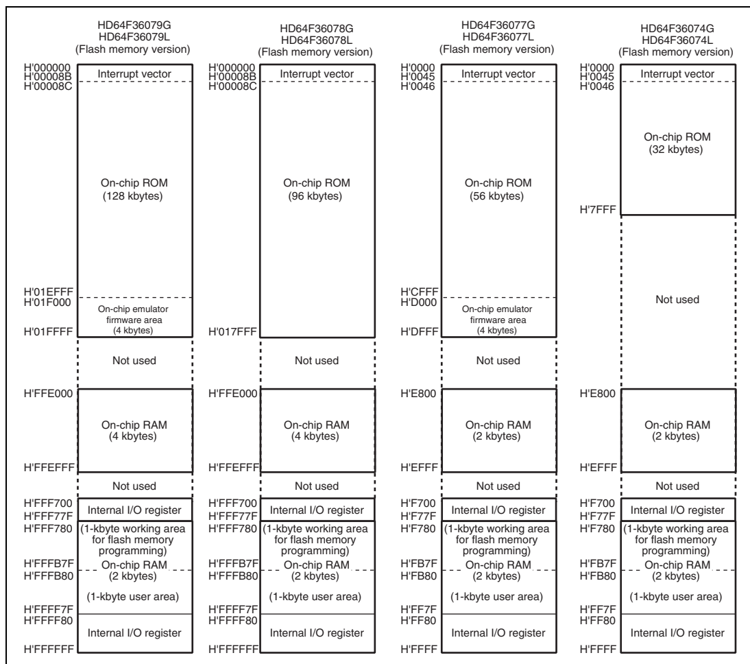
Figure 2.1 Memory Map
