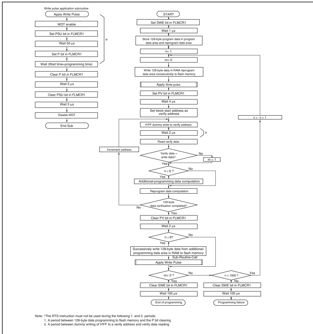
Figure 7.3 Program/Program-Verify Flowchart
