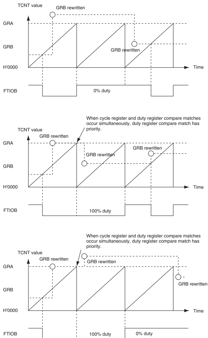
Figure 13.24 Example of PWM Mode Operation (3)
