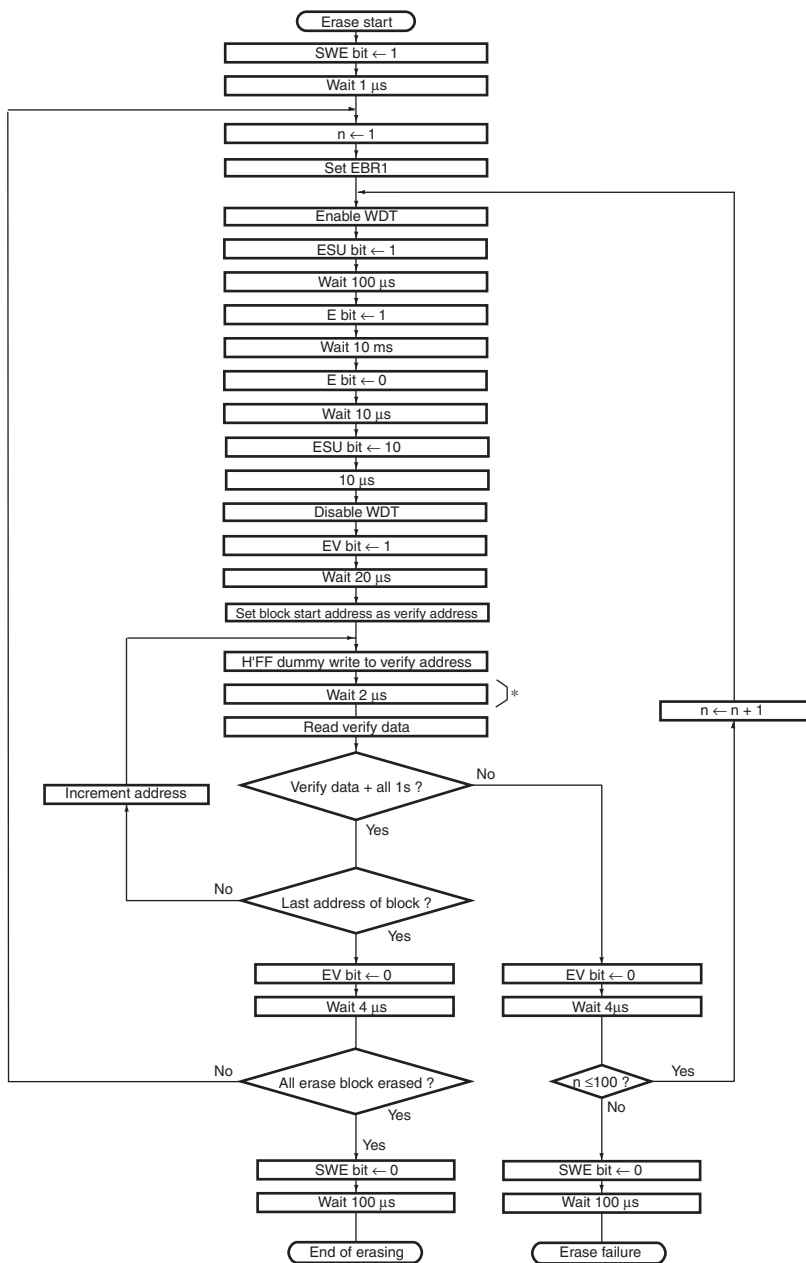
Figure 7.4 Erase/Erase-Verify Flowchart
