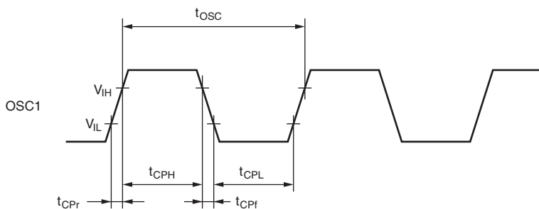
Figure 22.1 System Clock Input Timing
