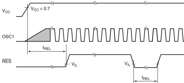
Figure 22.2 \overline{\text{RES}} Low Width Timing
