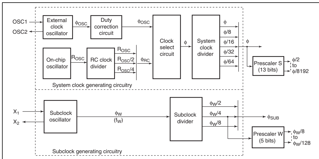
Figure 5.1 Block Diagram of Clock Pulse Generator
