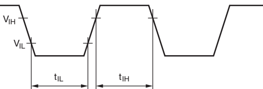
Figure 22.3 Input Timing
