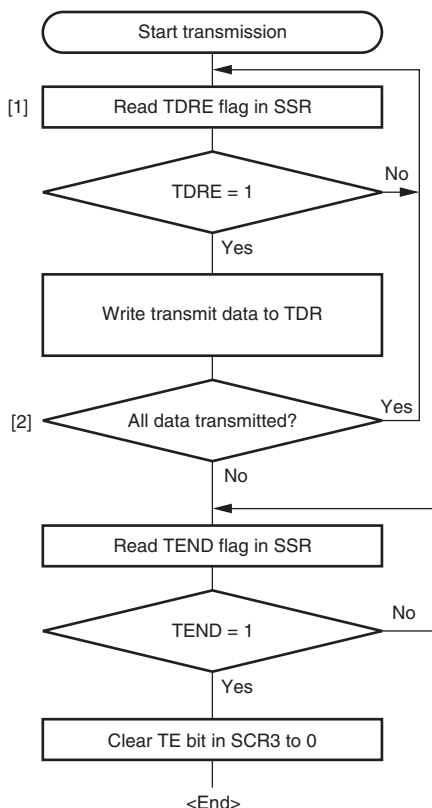
Figure 16.11 Sample Serial Transmission Flowchart (Clock Synchronous Mode)
