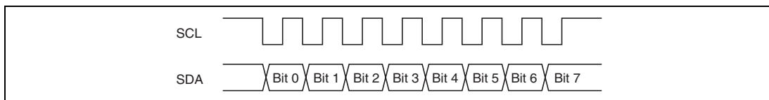
Figure 17.13 Clock Synchronous Serial Transfer Format
