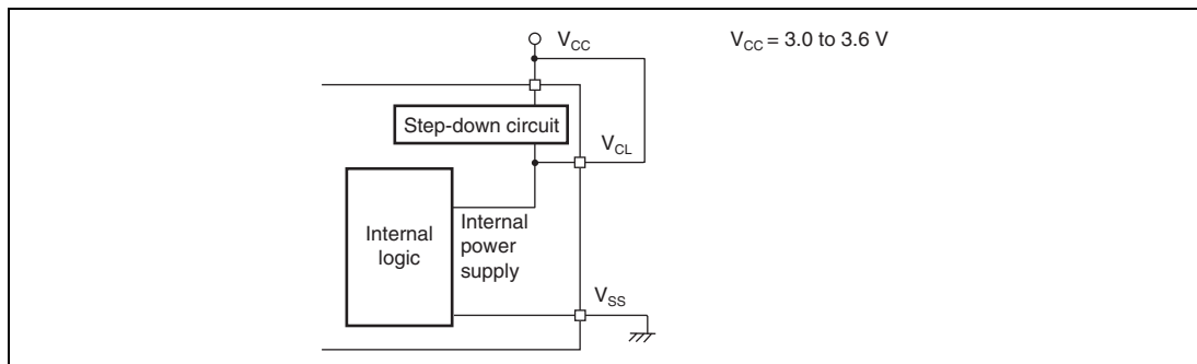
Figure 20.2 Power Supply Connection of 3.3-V-Specification Microcontrollers
