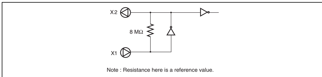
Figure 5.16 Block Diagram of Subclock Oscillator
