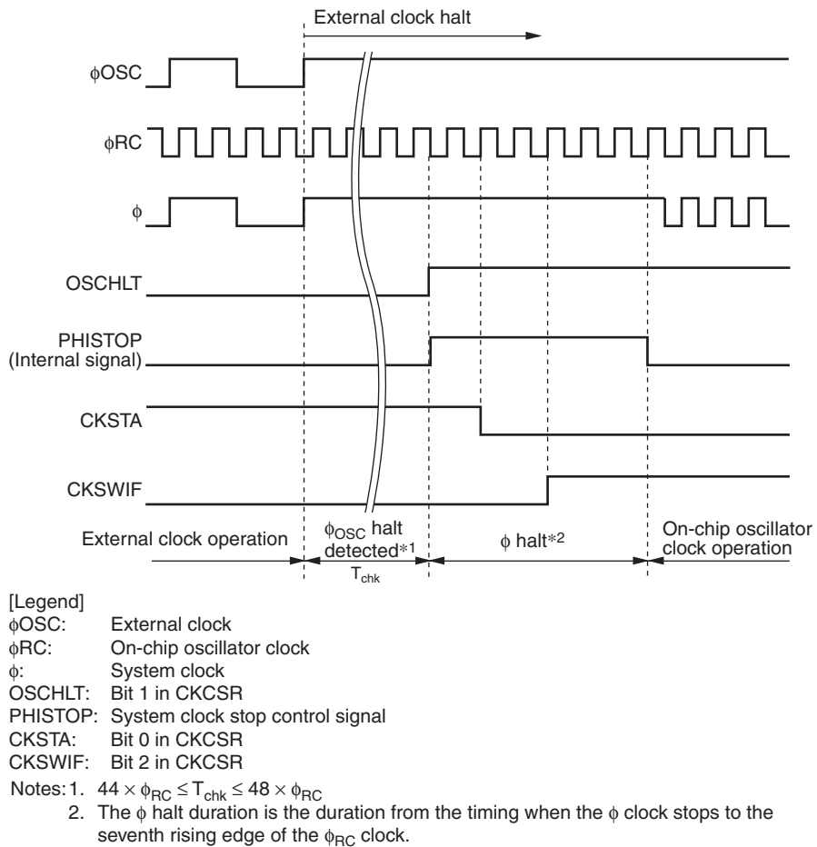
Figure 5.8 External Oscillation Backup Timing
