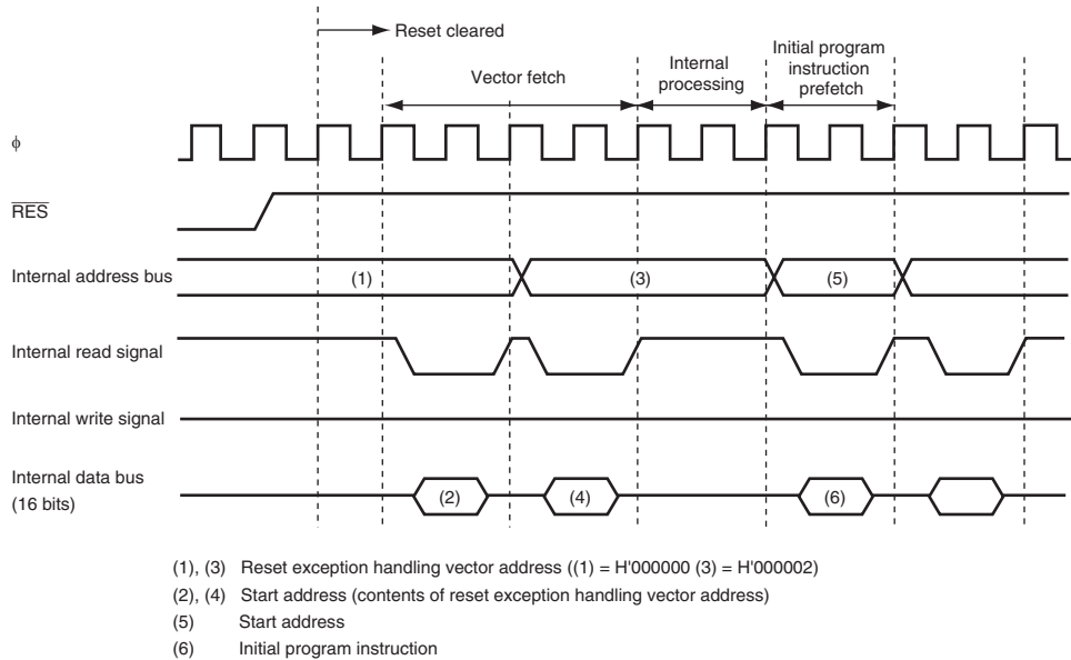
Figure 3.1 Reset Sequence
