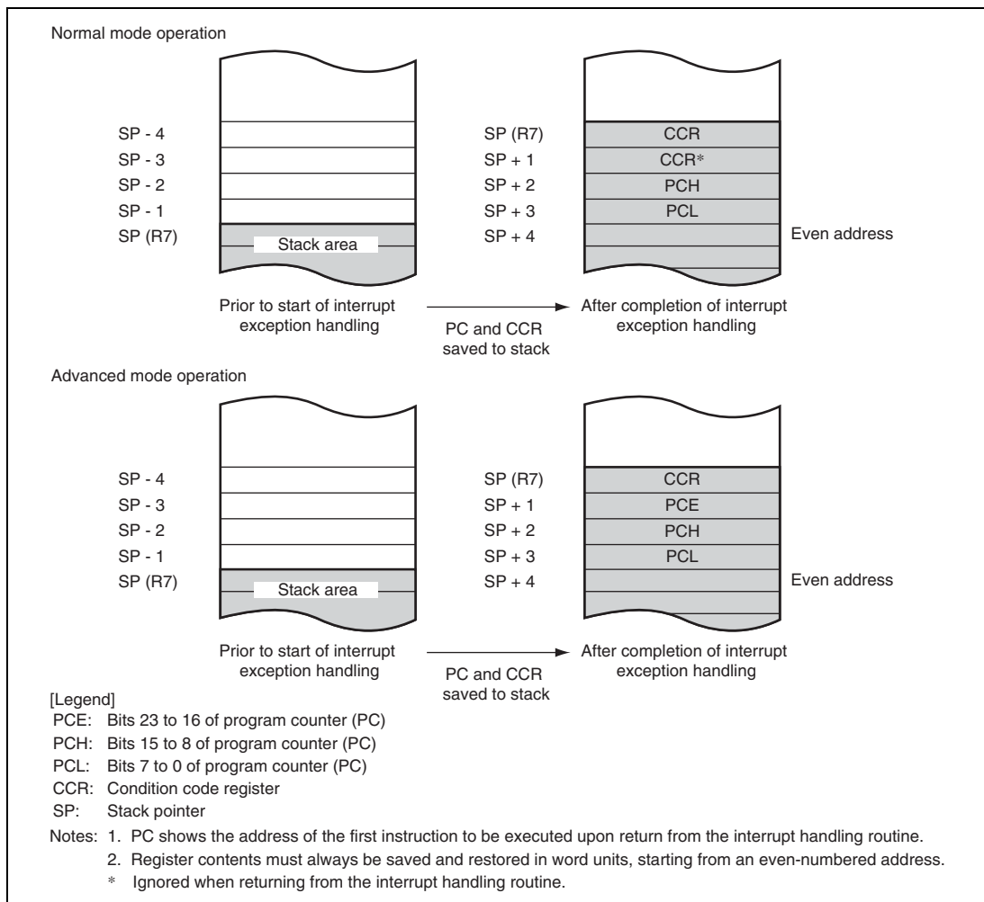
Figure 3.2 Stack Status after Exception Handling
