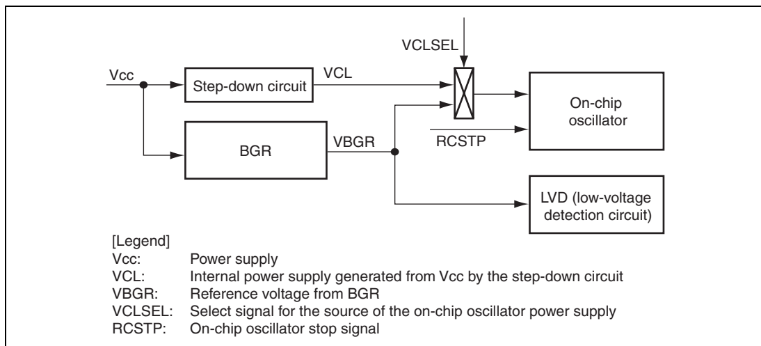
Figure 19.1 Block Diagram around BGR
