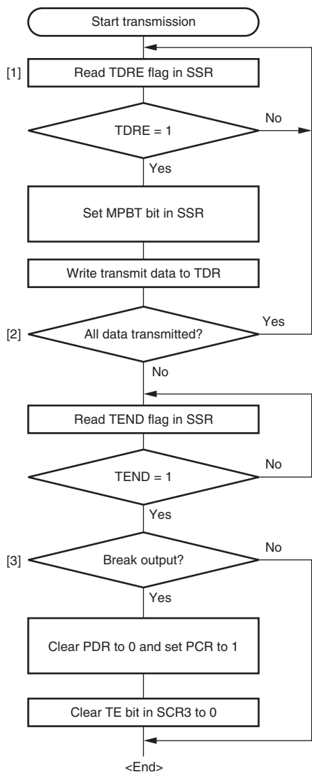
Figure 16.16 Sample Multiprocessor Serial Transmission Flowchart
