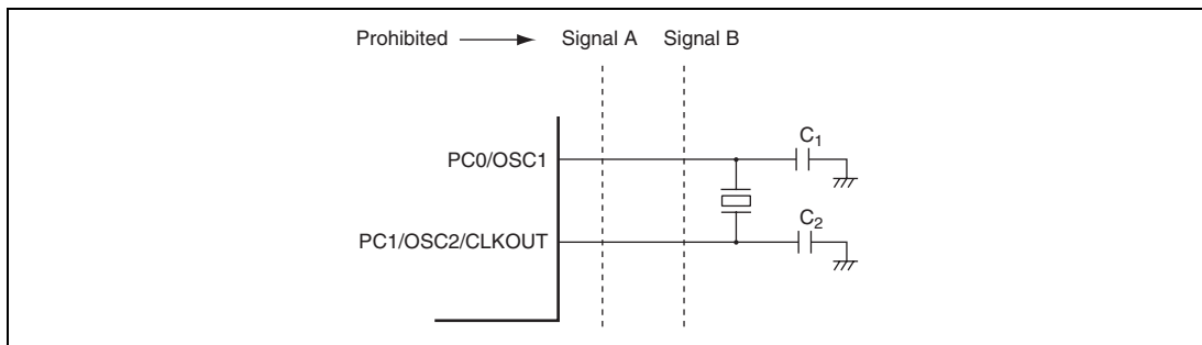
Figure 5.20 Example of Incorrect Board Design
