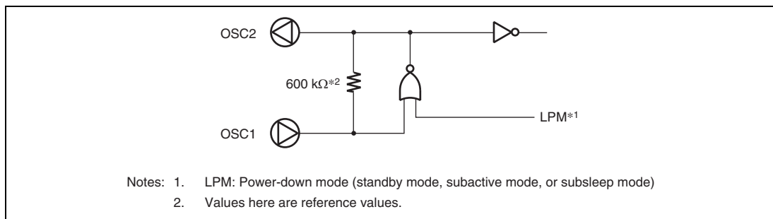
Figure 5.11 Block Diagram of External Clock Oscillator
