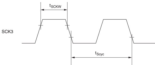
Figure 22.5 SCK3 Input Clock Timing
