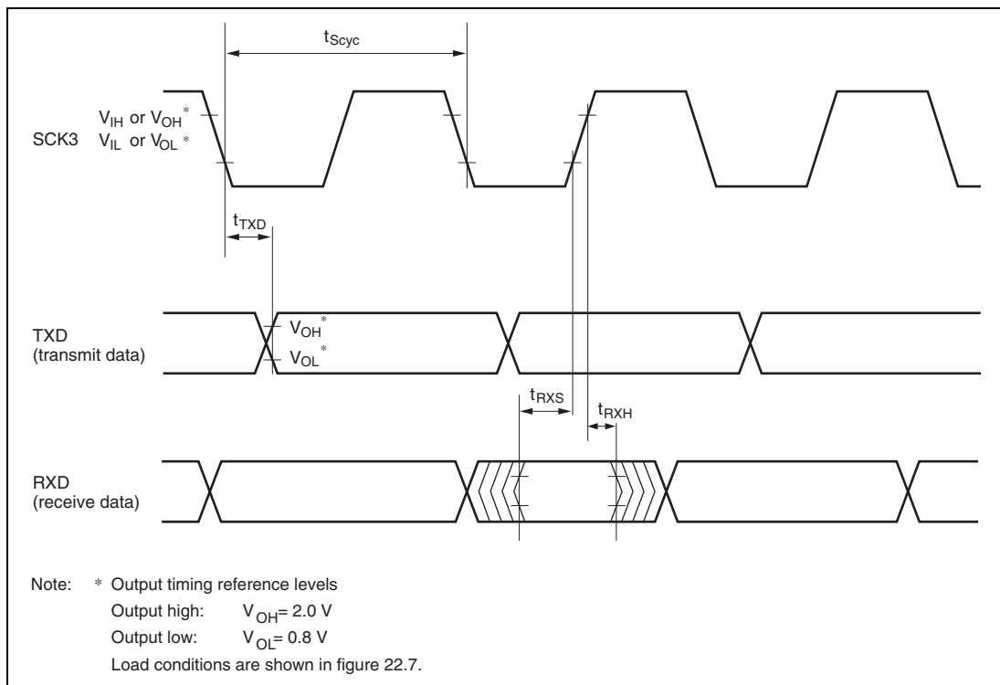
Figure 22.6 SCI Input/Output Timing in Clock Synchronous Mode
