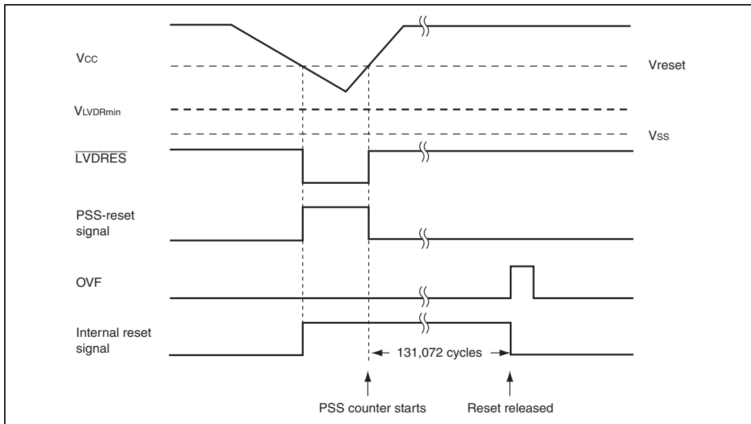
Figure 19.4 Operating Timing of LVDR Circuit
