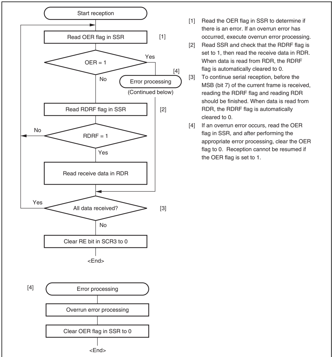
Figure 16.13 Sample Serial Reception Flowchart (Clock Synchronous Mode)
