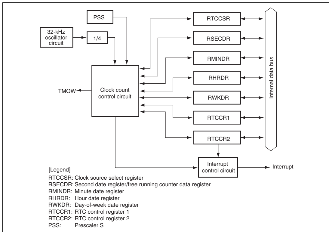
Figure 10.1 Block Diagram of RTC
