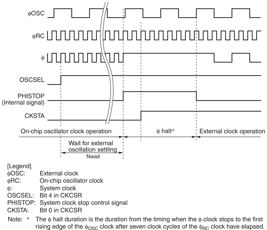
Figure 5.6 Timing Chart of Switching from On-Chip Oscillator Clock to External Clock
