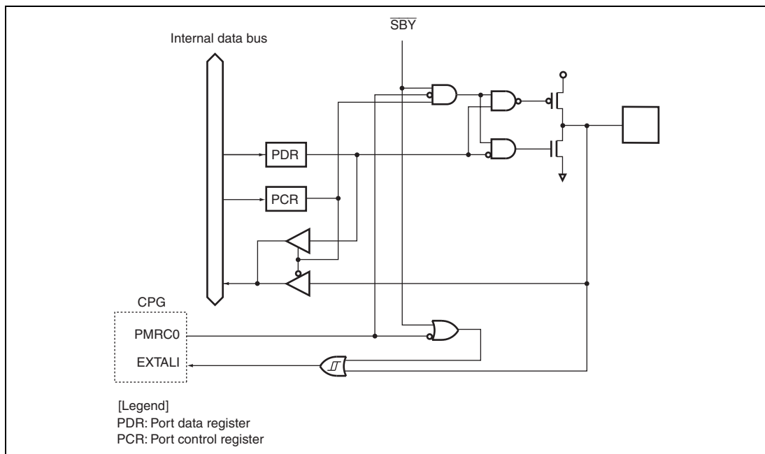
Figure B.26 Port B Block Diagram (PC0)
