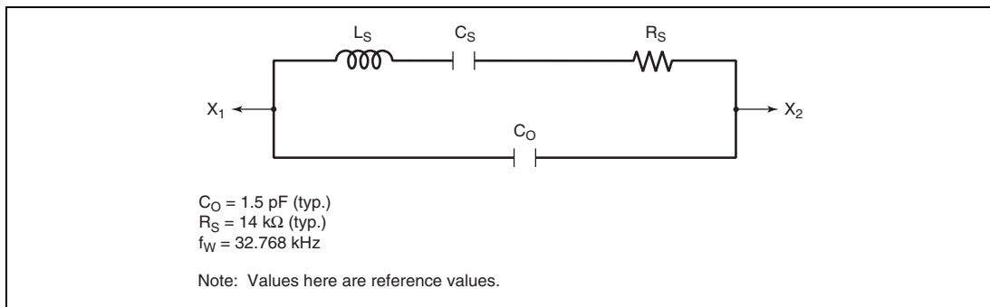
Figure 5.18 Equivalent Circuit of 32.768-kHz Crystal Resonator
