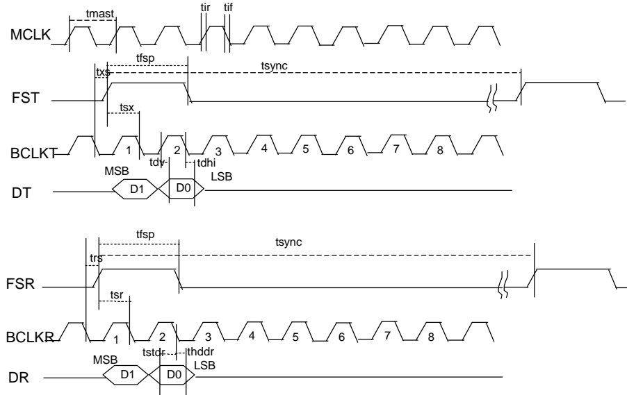
Figure 9-1 Long Frame Sync, Timing
