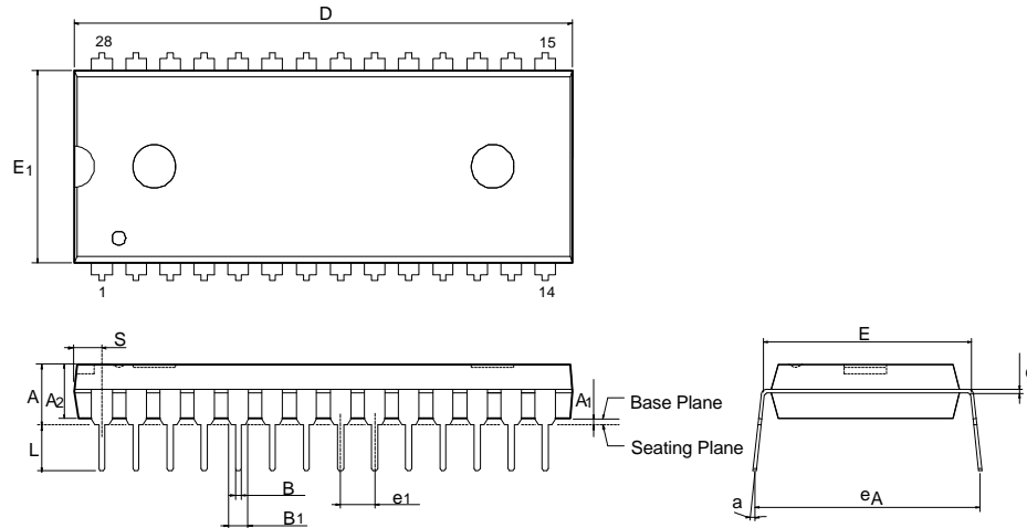
Figure12-2 28-Lead Plastic DIP Package
