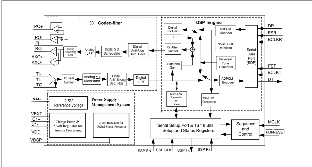
Figure 6-1 Winbond ADPCM ΣΔ Codec Block Diagram
