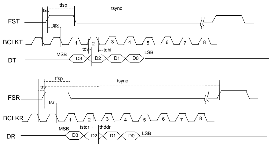
Figure 9-2 Short Frame Sync, Timing
