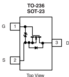
SQ7002K (8K)* * Marking Code 8K
