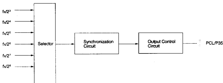
Figure 5-4. Clock Output Control Circuit Block Diagram
