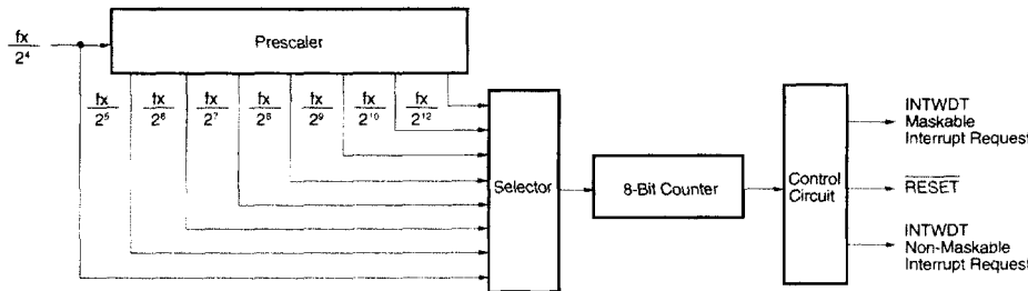
Figure 5-3. Watchdog Timer Block Diagram
