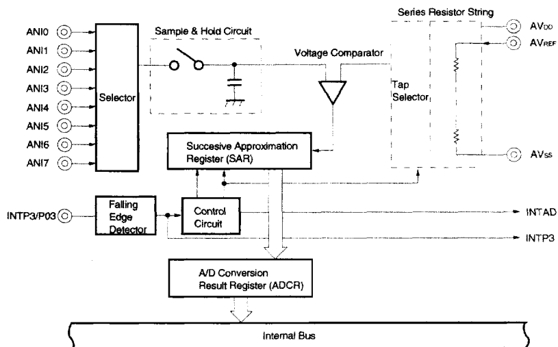
Figure 5-6. A/D Converter Block Diagram
