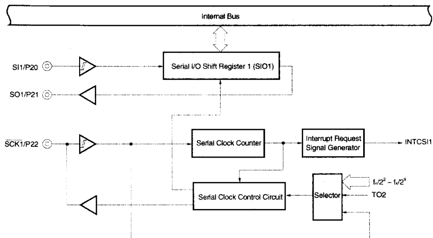
Figure 5-7. Serial Interface Channel 1 Block Diagram
