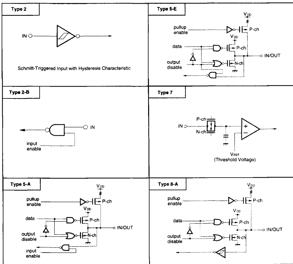
Figure 3-1. Pin Input/Output Circuits
