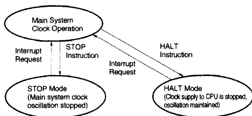
Figure 7-1. Standby Functions
