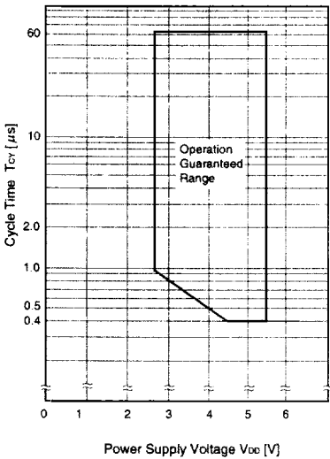
TCY vs VDD (Main System Clock Operation)
