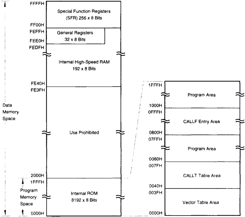
Figure 4-1. Memory Map
