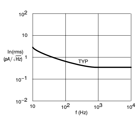
Figure 11. Input Noise Current Density
