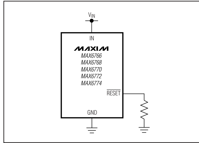
Figure 5. Ensuring \overline{\text{RESET}} Valid to V_{IN} = 0V
