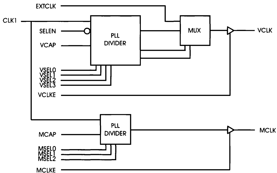
Figure 2-2 ICS90C64A Functional Block Diagram
