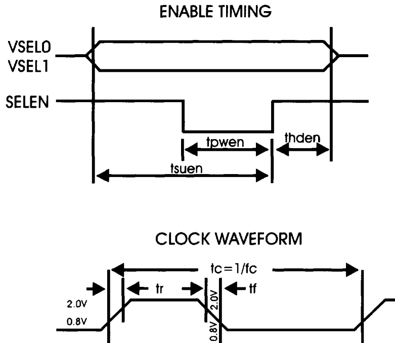
Figure 5-1 ICS90C64A Timing
