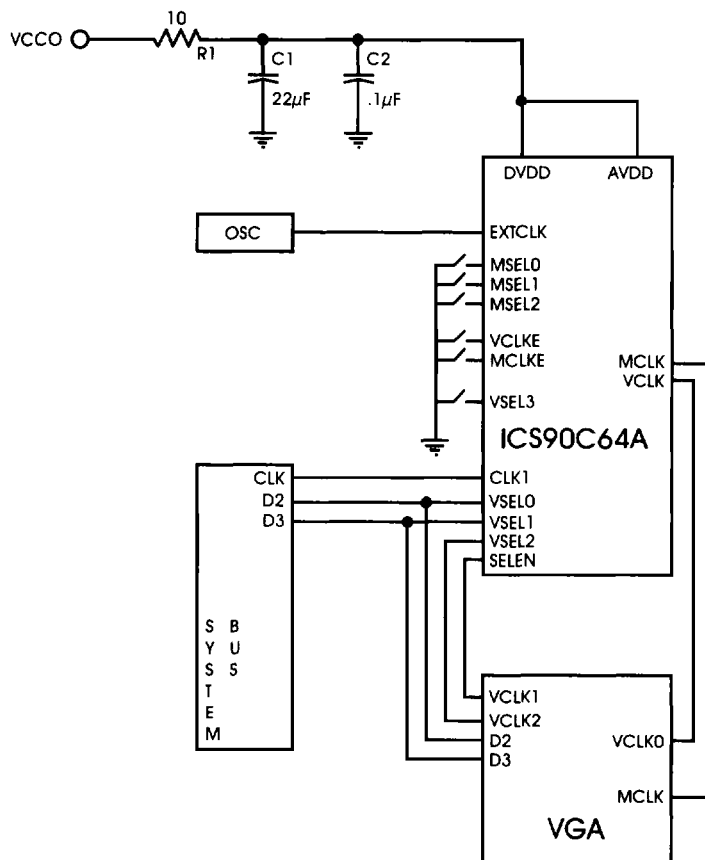
Figure 2-1 ICS90C64A Interface
