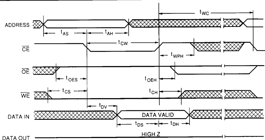
FIGURE 4. \overline{\text{CE}} CONTROLLED WRITE CYCLE TIMING
