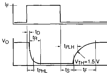
Figure 6. Switching timing
