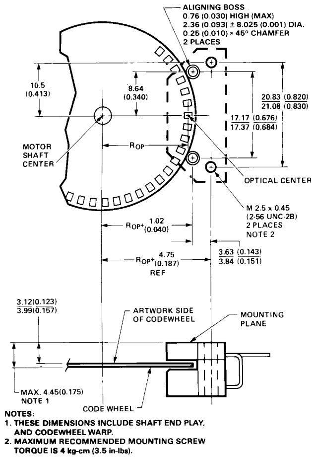
Figure 2. Mounting Plane Side A.
