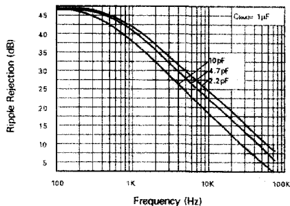
Ripple Rejection vs. Frequency
