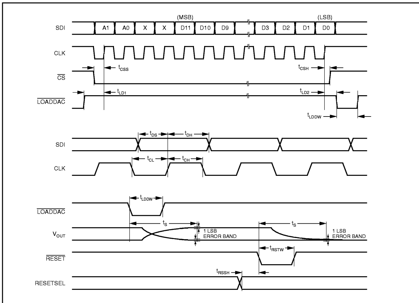
FIGURE 3. DAC7614 Timing.
