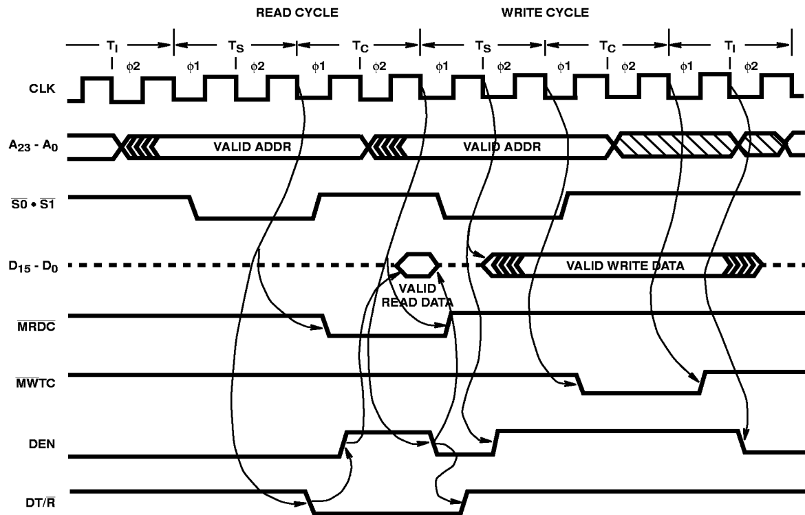
FIGURE 25. BACK TO BACK READ-WRITE CYCLE
