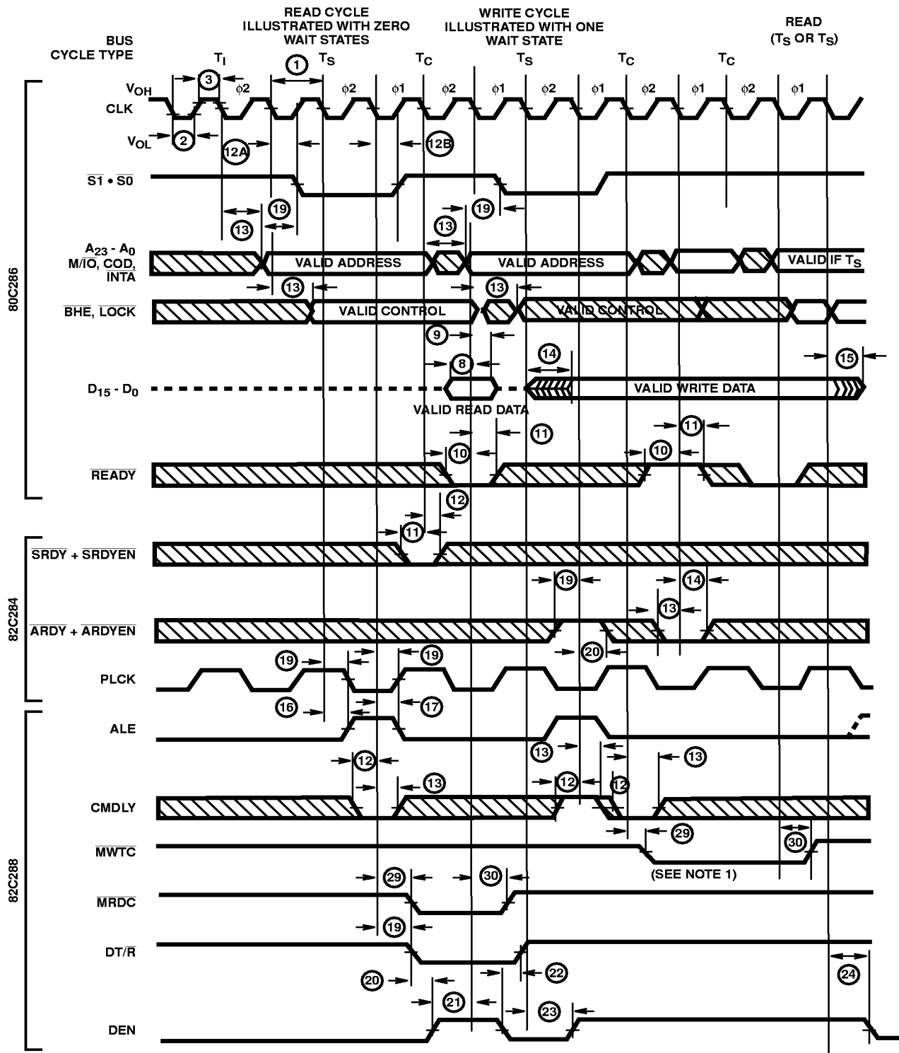
FIGURE 34. MAJOR CYCLE TIMING
