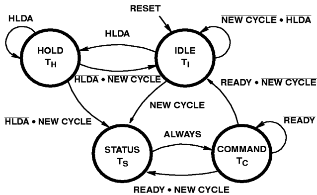
FIGURE 21. 80C286 BUS STATES
