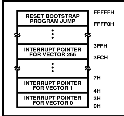
FIGURE 7. 80C286 REAL ADDRESS MODE INITIALLY RESERVED MEMORY LOCATIONS
