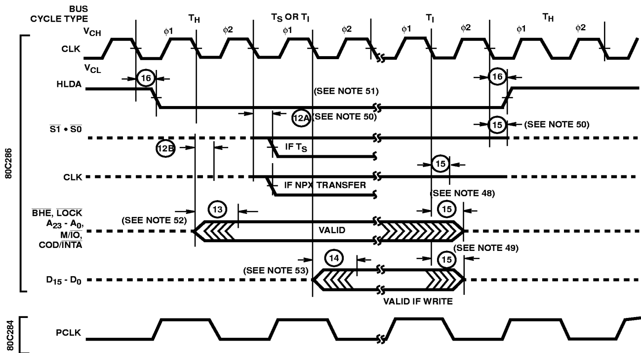
FIGURE 37. EXITING AND ENTERING HOLD
