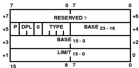
FIGURE 10. SYSTEM SEGMENT DESCRIPTOR
