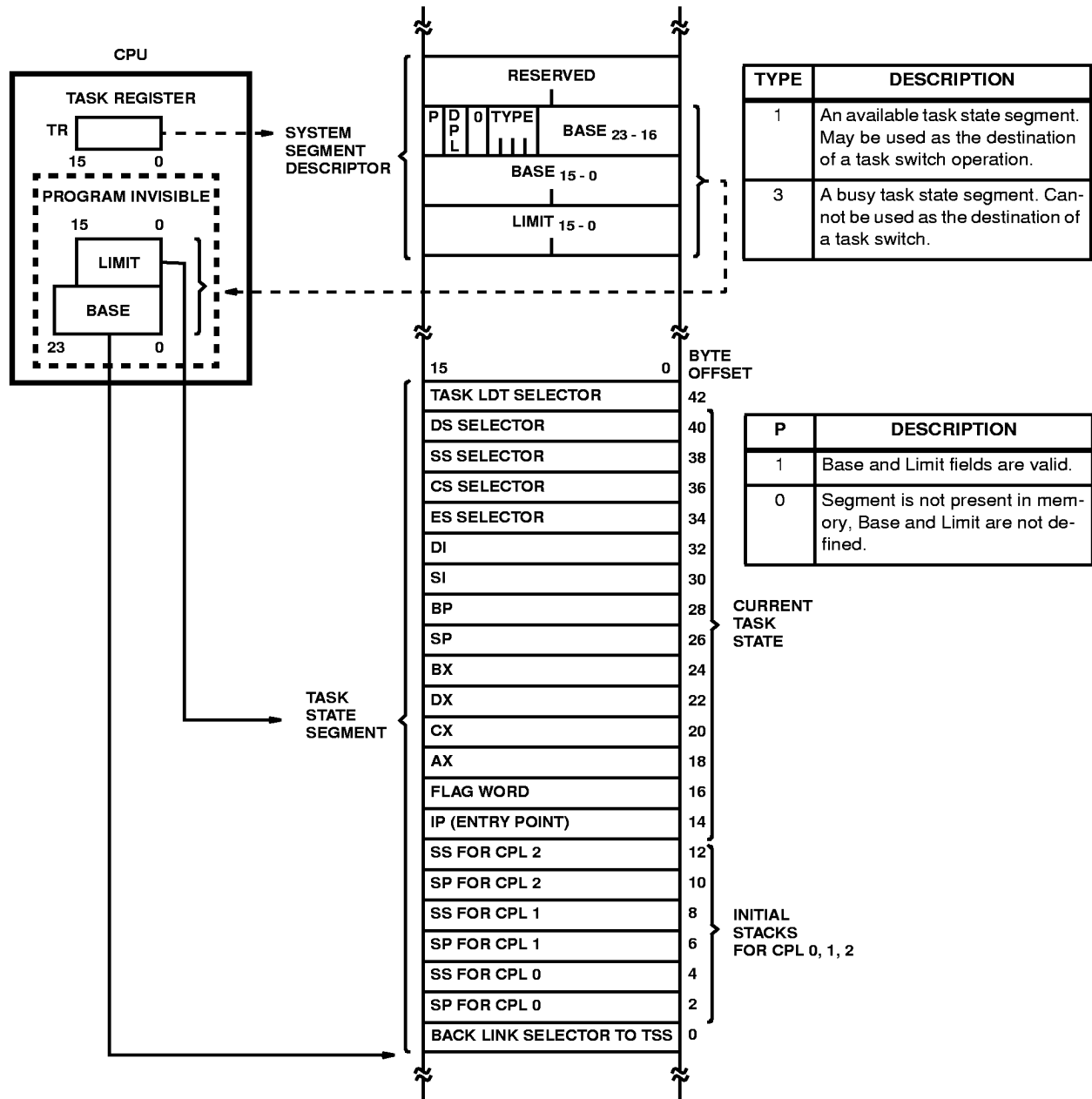
FIGURE 18. TASK STATE SEGMENT AND TSS REGISTERS
