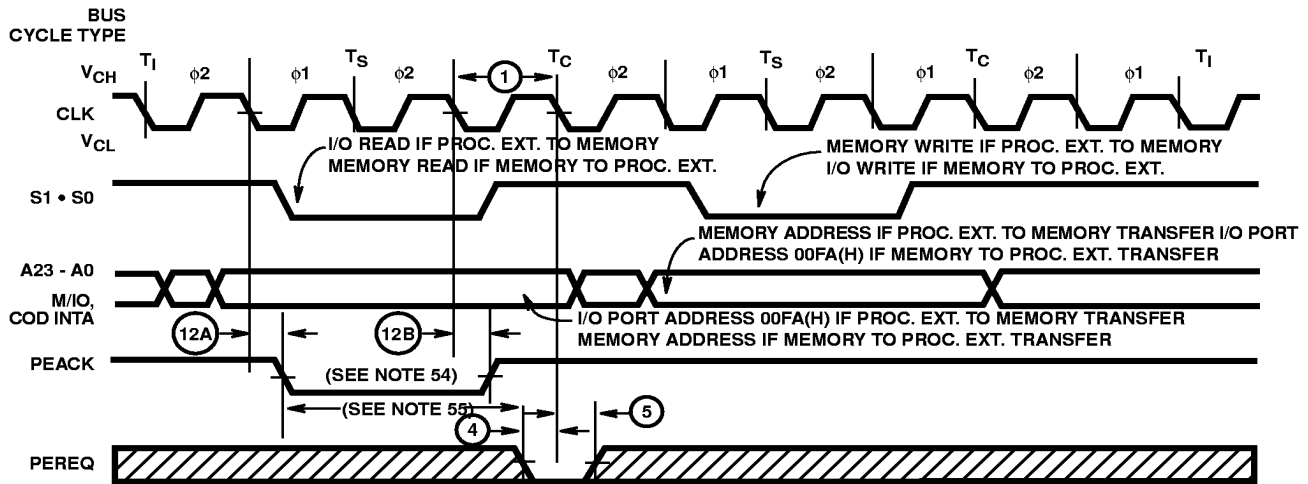
FIGURE 38. 80C286 PEREQ/PEACK TIMING FOR ONE TRANSFER ONLY
