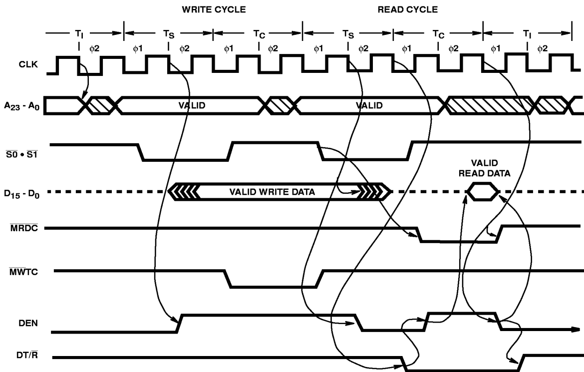
FIGURE 26. BACK TO BACK WRITE-READ CYCLE
