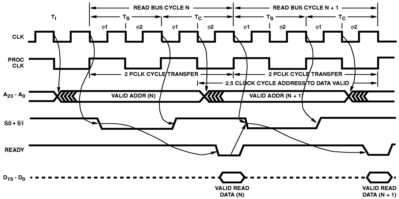
FIGURE 22. BASIC BUS CYCLE
