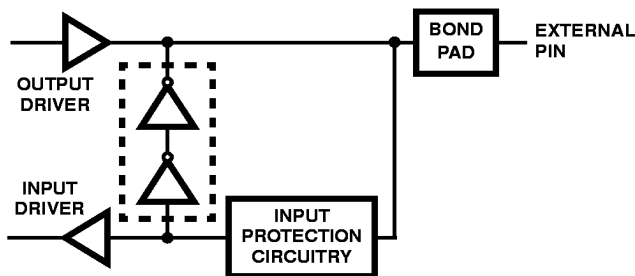
FIGURE 19A. BUS HOLD CIRCUITRY, PINS 36-51, 66, 67
