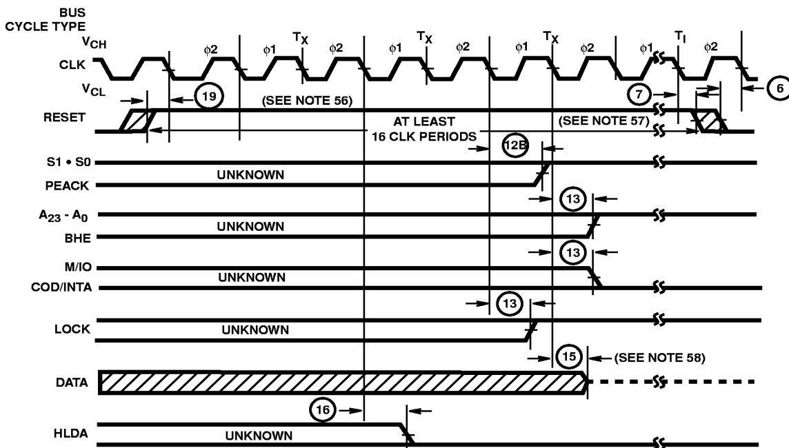
FIGURE 39. INITIAL 80C286 PIN STATE DURING RESET
