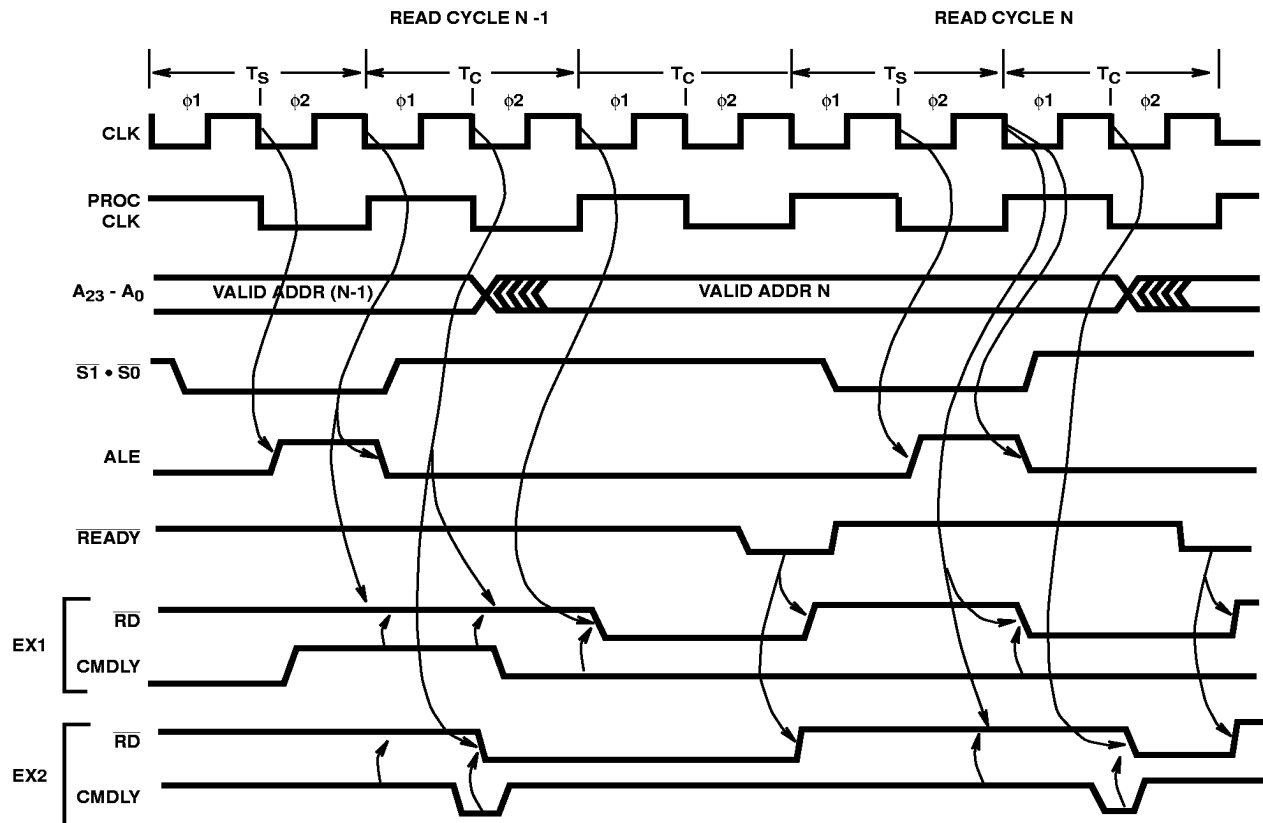
FIGURE 23. CMDLY CONTROLS THE LEADING EDGE OF COMMAND SIGNAL
