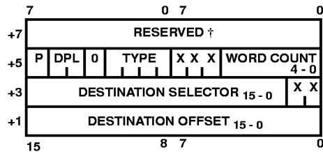
FIGURE 11. GATE DESCRIPTOR
