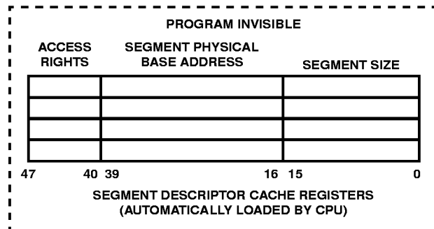
FIGURE 12. DESCRIPTOR CACHE REGISTERS
