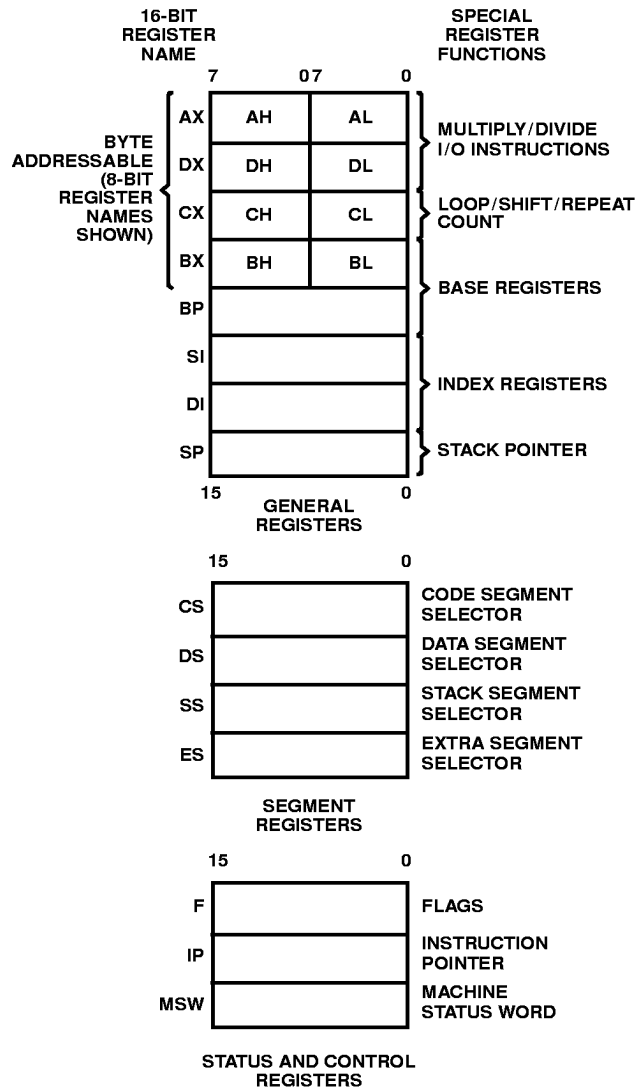
FIGURE 1. REGISTER SET
