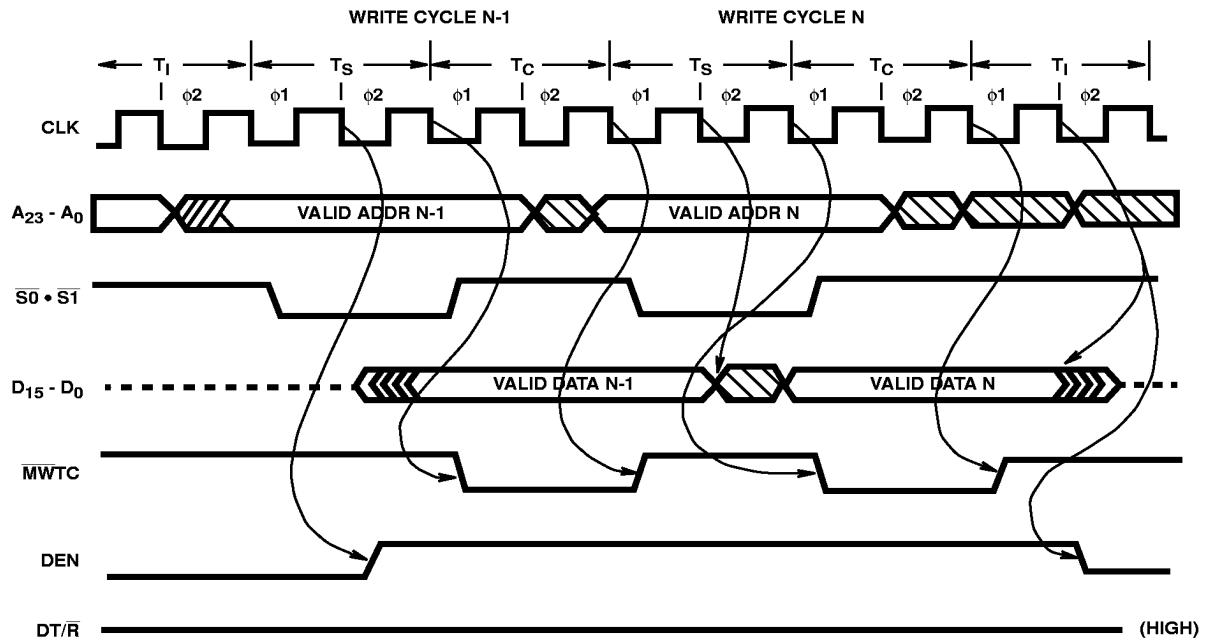
FIGURE 27. BACK TO BACK WRITE-WRITE CYCLE
