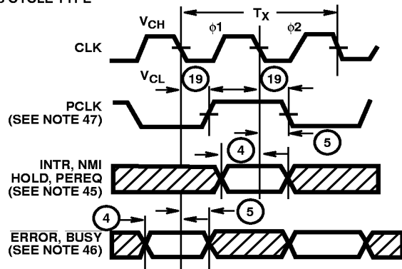
FIGURE 35. 80C286 ASYNCHRONOUS INPUT SIGNAL TIMING NOTES:
