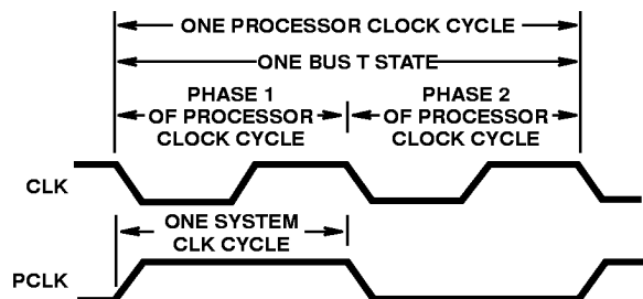
FIGURE 20. SYSTEM AND PROCESSOR CLOCK RELATIONSHIPS
