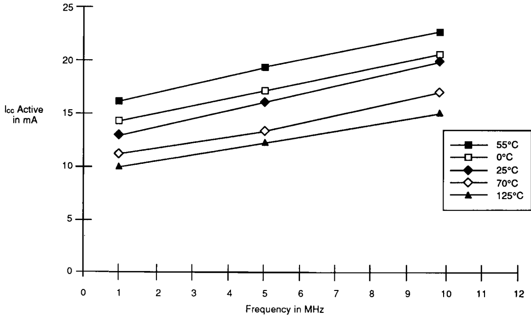
Figure 5. Am28F010—Average Icc Active vs. Frequency
