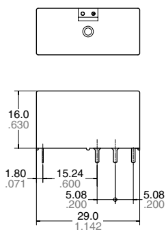
Single side stable type 1 coil latching type 2 coil latching type
