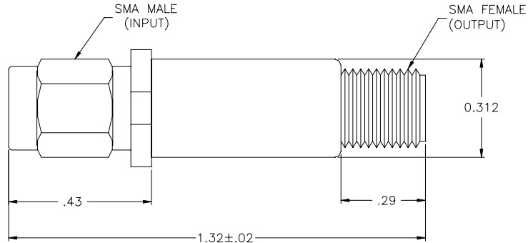
STANDARD CASE STYLE C3 (Optional Case Styles – C36, C37, M22)
