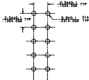
RECOMMENDED MOUNTING HOLE LAYOUT
