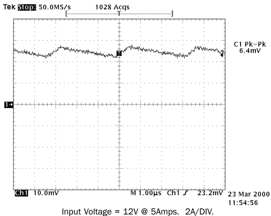
Figure 7: Output Current
