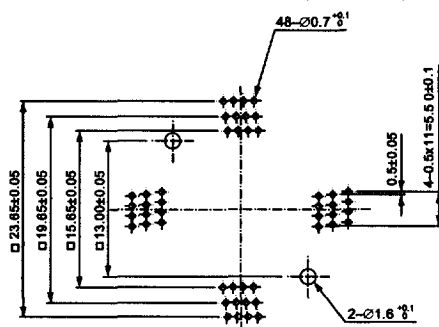
QFP IC234-0484-034 (48 Pins)
