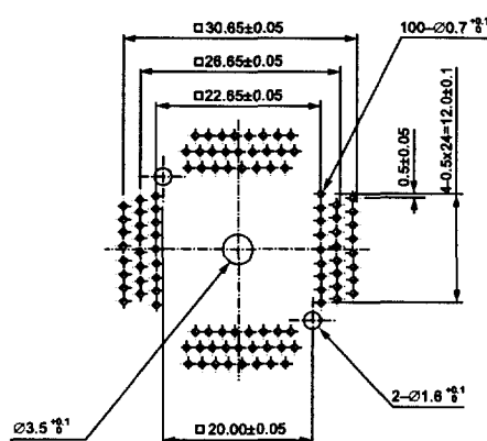
QFP IC234-1004-023 (100 Pins)
