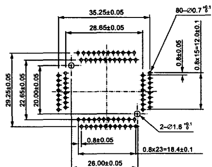
QFP IC234-0804-001 (80 Pins)
