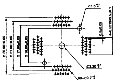
QFP IC234-0804-001 (80 Pins)
