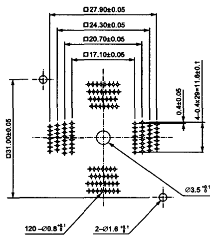
QFP IC234-1204-022 (120 Pins)
