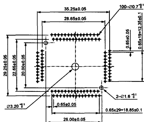
QFP IC234-1004-033 (100 Pins)
