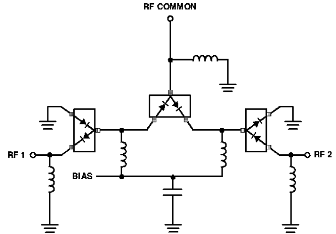
Figure 18. Very High Isolation SPDT Switch.
