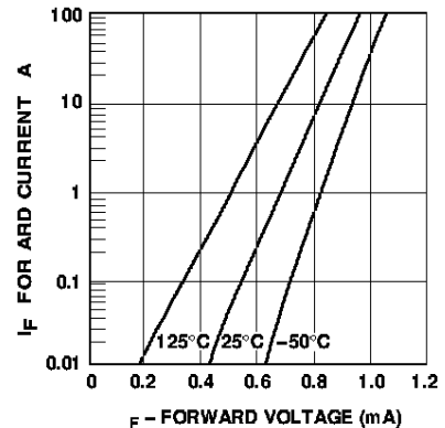
Figure 12. Forward Current vs. Forward Voltage. HSMP-482B.
