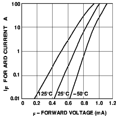
Figure 11. Forward Current vs. Forward Voltage. HSMP-381B/C/E/F Series and HSMP-481B.
