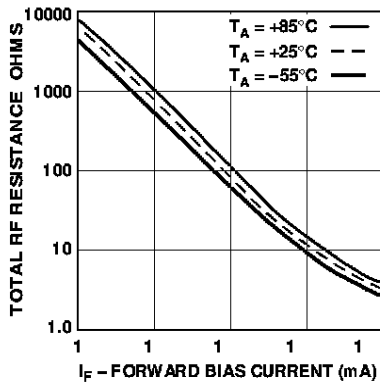
Figure 4. RF Resistance vs. Forward Bias Current for HSMP-381B/C/E/F Series and HSMP-481B.
