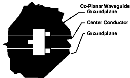
Figure 25. Circuit Layout.
