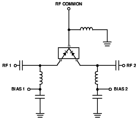
Figure 15. Simple SPDT Switch, Using Only Positive Bias Current.
