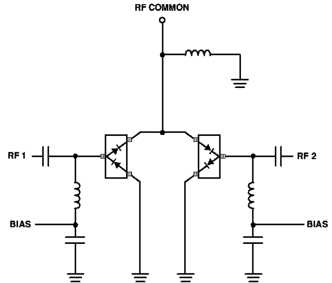
Figure 16. High Isolation SPDT Switch.
