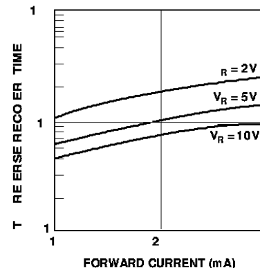
Figure 8. Reverse Recovery Time vs. Forward Current for Various Reverse Voltages. HSMP-482B.
