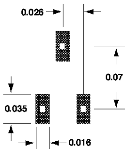
Figure 27. PCB Pad Layout (dimensions in inches).
