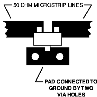
Figure 23. Circuit Layout.
