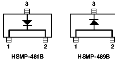
Figure 21. Internal Connections.
