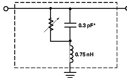
Figure 26. Equivalent Circuit.
