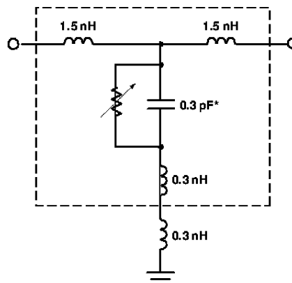
Figure 24. Equivalent Circuit.
