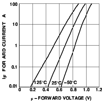
Figure 13. Forward Current vs. Forward Voltage. HSMP-386B/C/E/F Series.
