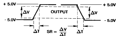
OVERSHOOT, RISE & FALL TIME WAVEFORMS
