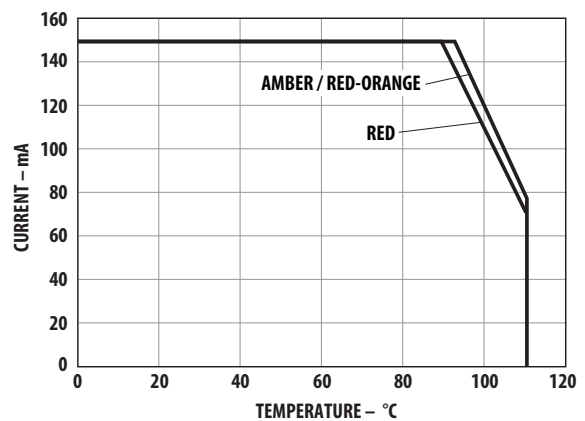
Figure 6b. Maximum forward current vs. solder point temperature. Derated based on T_{JMAX} = 125^{\circ}\text{C} , R_{JP} = 60^{\circ}\text{C/W} .
