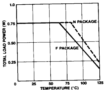
Total Load Power vs Temperature (NE590)
