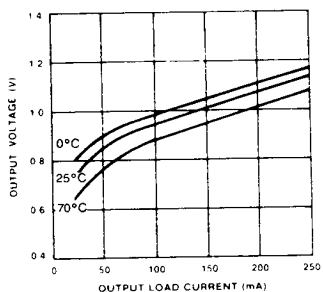
Output Voltage vs Load Current (NE590)
