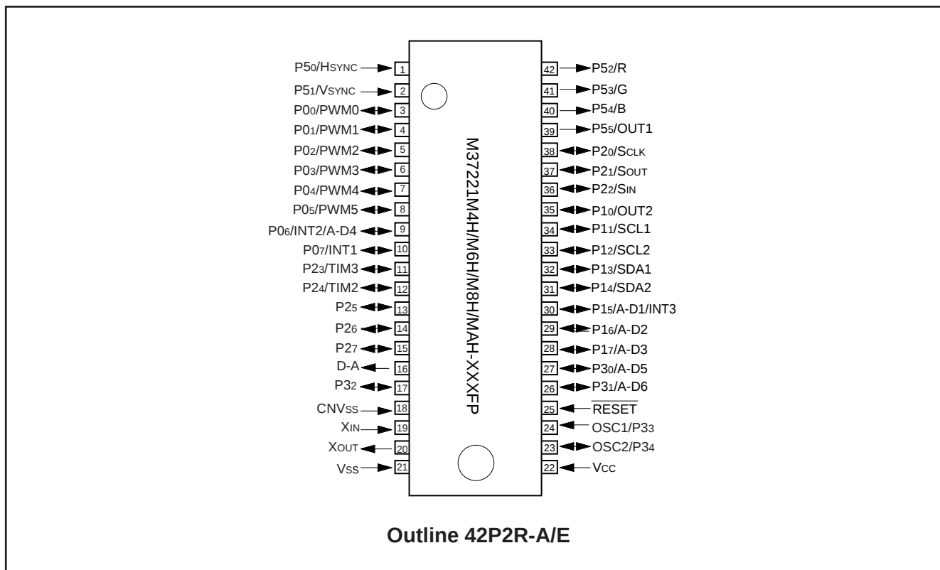
Fig. 4.2 Pin Configuration (2) (Top View)
