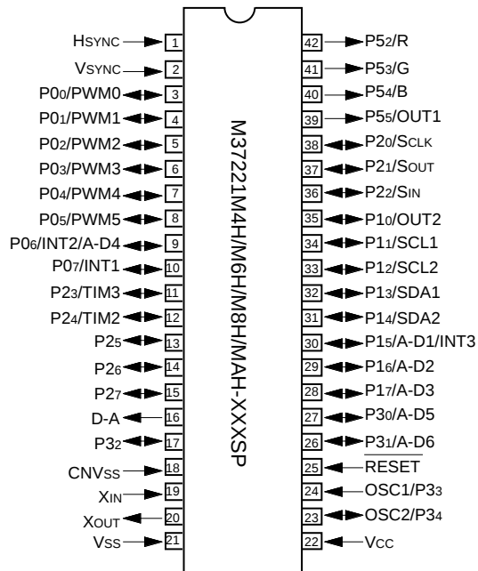
Outline 42P4B
