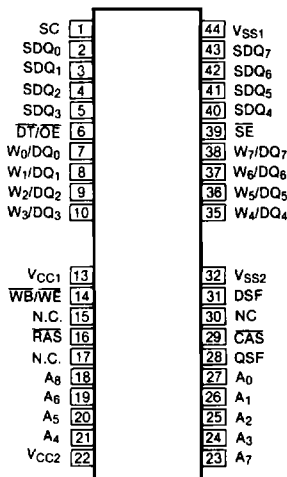
40/44 Pin 400 mil TSOP II
