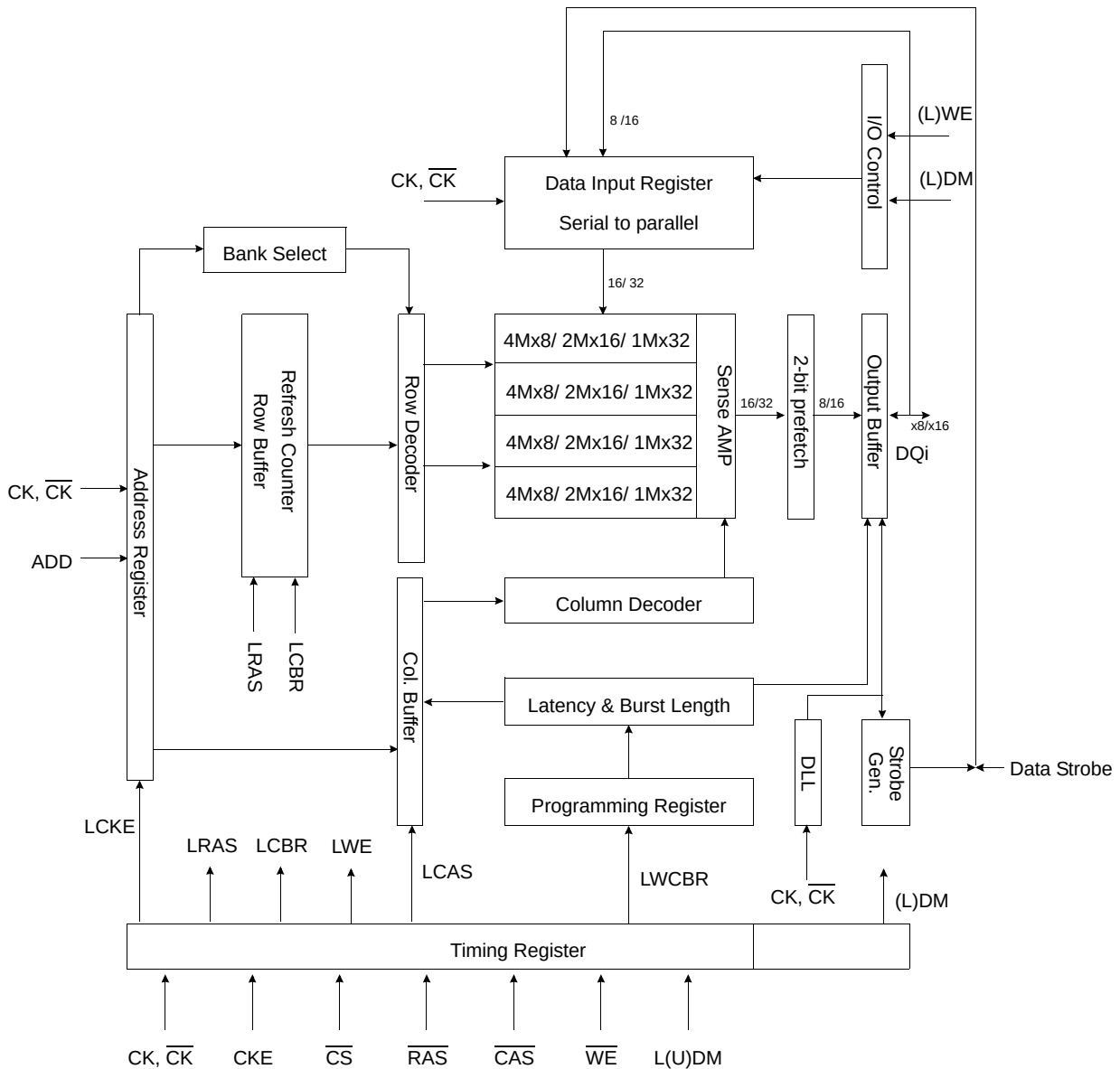
Block Diagram (8Mbit x 4 / 4Mbit x 8 / 2Mbit x 16 I/O x 4 Banks)
