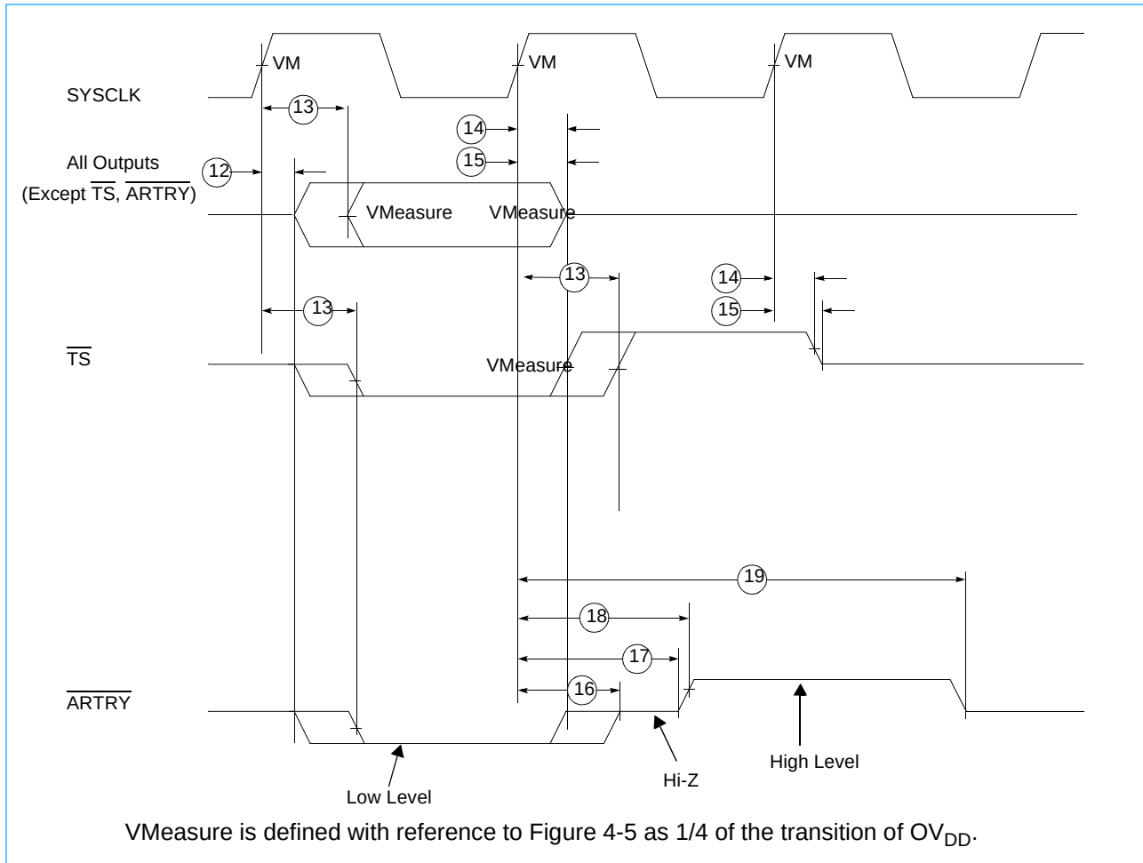
Figure 4-6. Output Timing Diagram for PowerPC 750Cxe
