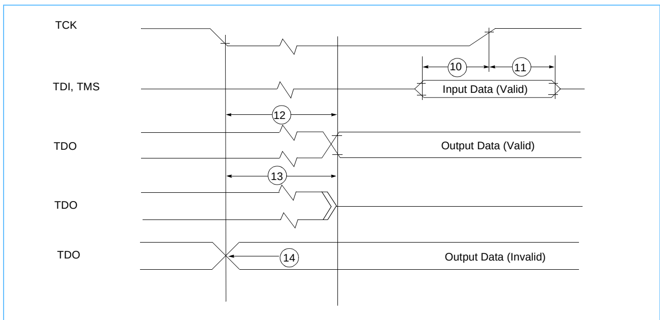
Figure 4-10. Test Access Port Timing Diagram
