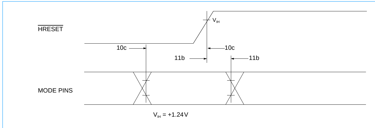
Figure 4-4. Mode Select Input Timing Diagram
