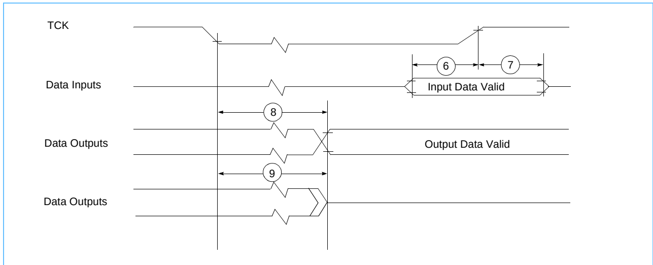
Figure 4-9. Boundary-Scan Timing Diagram
