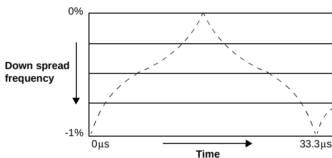
Figure 4-2. Linear Sweep Modulation Profile
