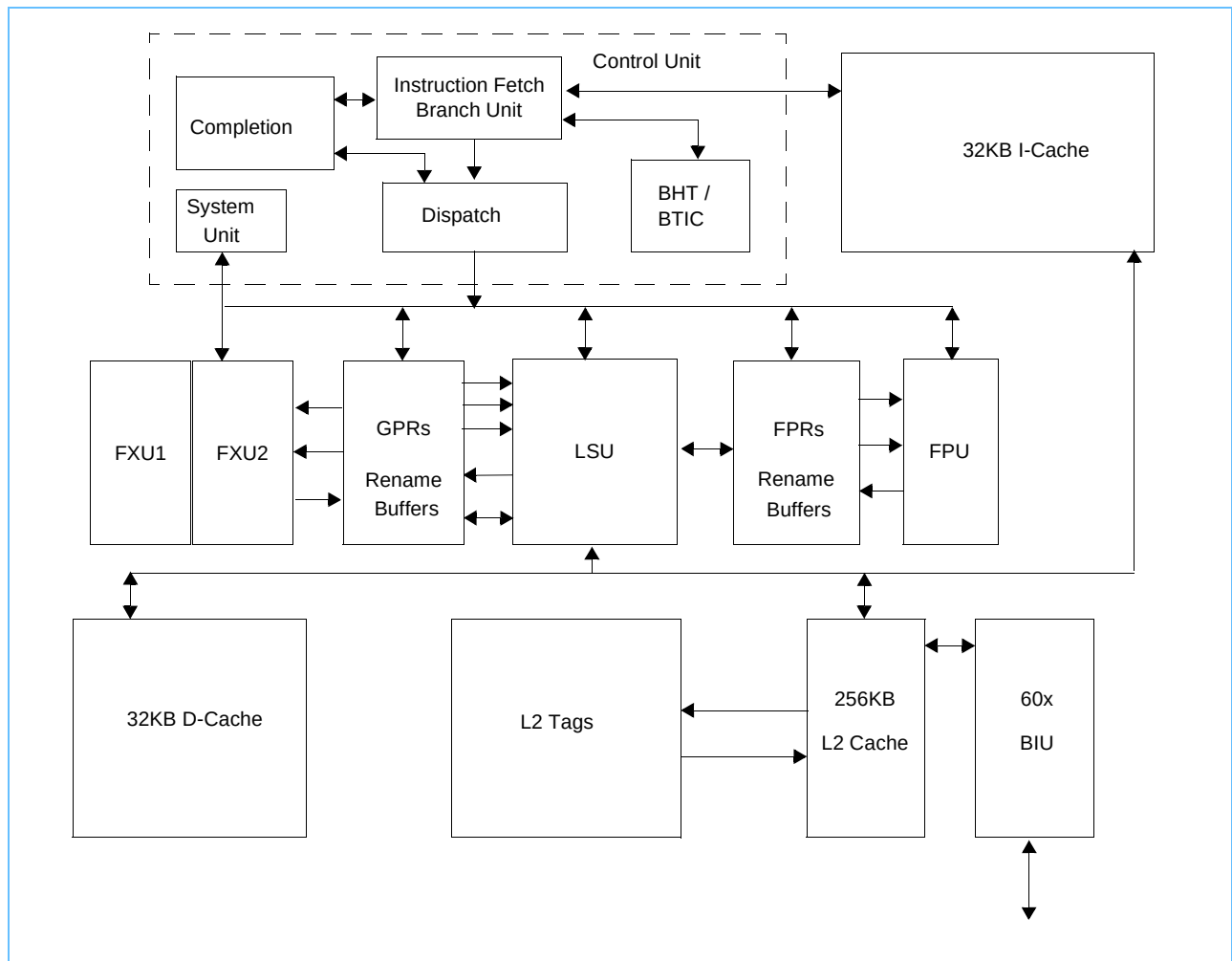
Figure 2-1. PowerPC 750Cxe Block Diagram
