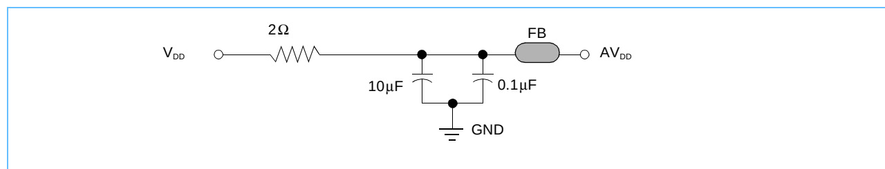
Figure 6-1. PLL Power Supply Filter Circuit
