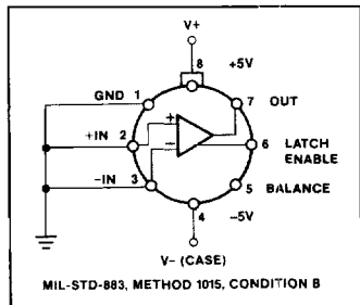
STANDARD BURN-IN CIRCUIT
