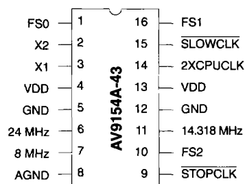
16-Pin PDIP or SOIC AV9154A-43 K-4, K-6
