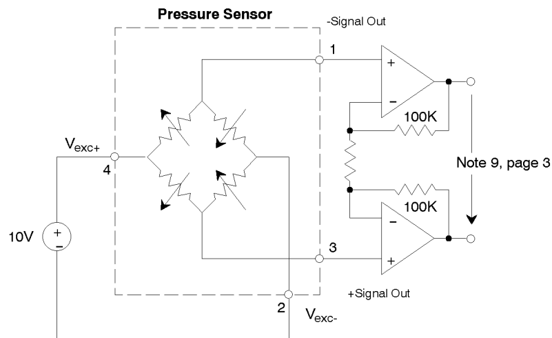
Figure 2. SM5612 and SM5652 with Constant Voltage Supply and Differential Output
