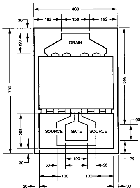
MGFC0904 OUTLINE DRAWING
