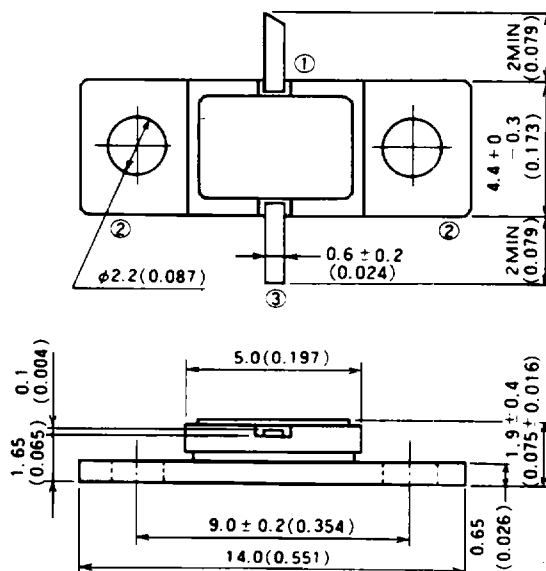
MGF0904A/MGF0905A OUTLINE DRAWING
