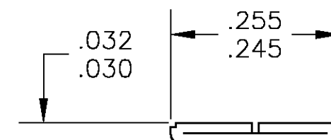
SECTION A-A SCALE 5:1
