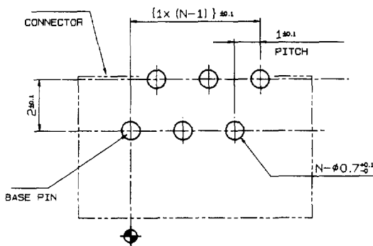
MOUNTING LAYOUT
