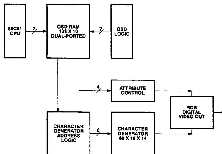
Figure 3. On-Screen Display (OSD) Block
