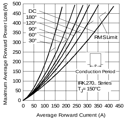
Fig. 15 - Forward Power Loss Characteristics
