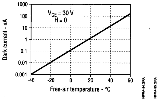
Fig. 3 Detector Dark Current vs Temperature
