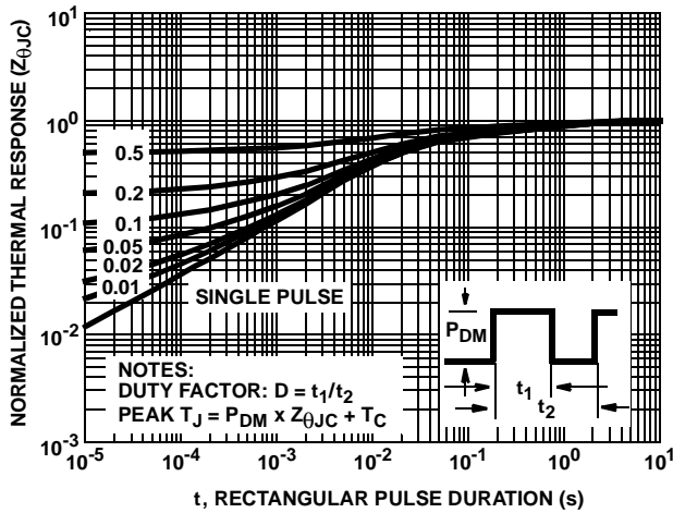
FIGURE 9. NORMALIZED MAXIMUM TRANSIENT THERMAL RESPONSE
