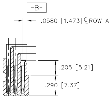
SECTION X-X
