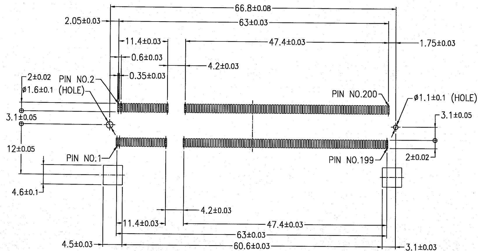
RECOMMENDED MOUNTING P.C.B LAYOUT
