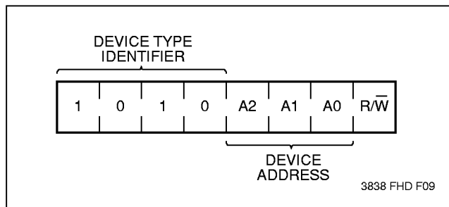
Figure 4. Slave Address
