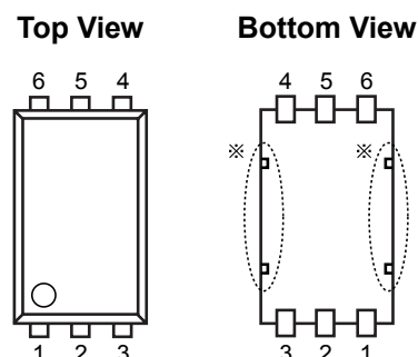
SON-6
