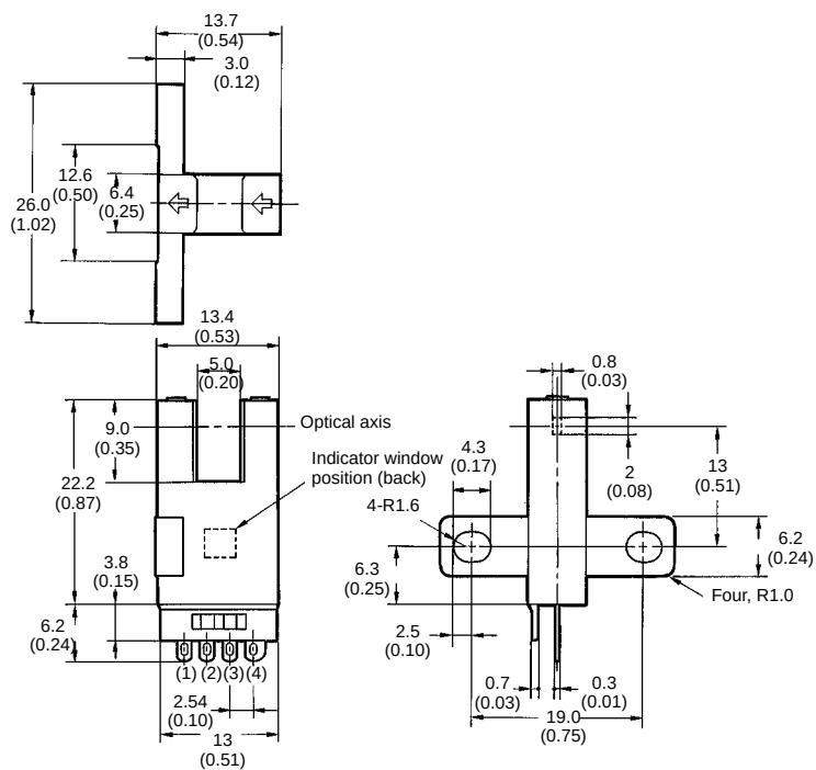
Terminal Arrangement
