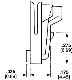
Latch
