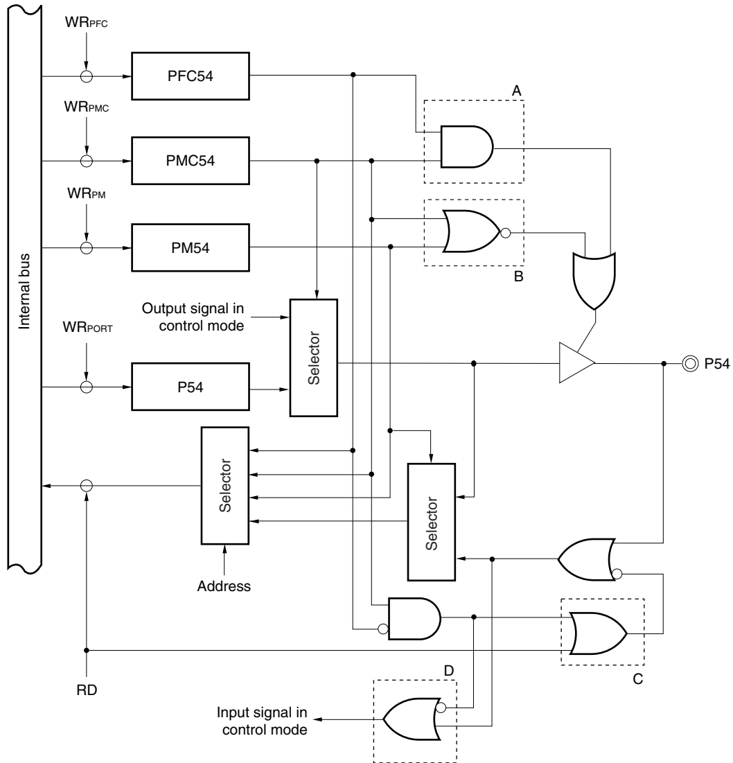
Figure 14-10. Block Diagram of Type G-1
