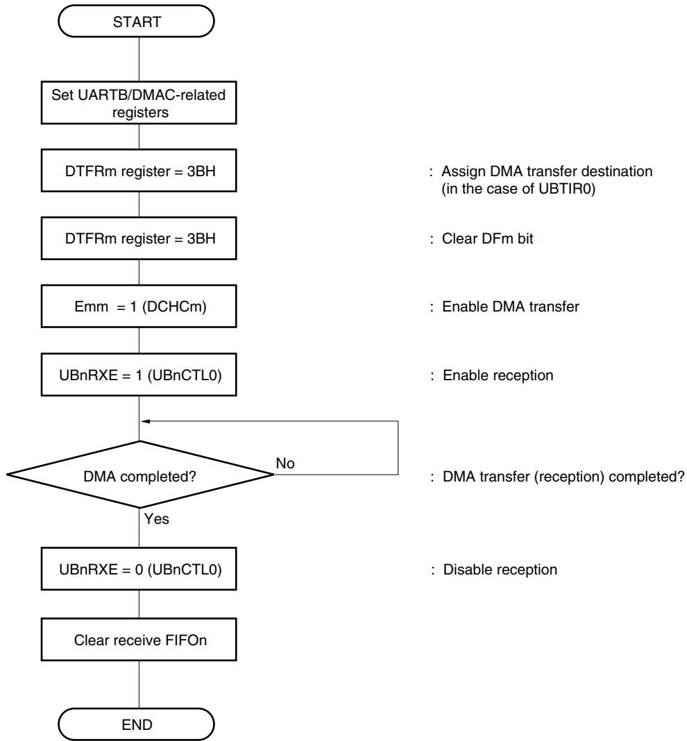
Figure 10-18. Example of Continuous Reception (Pending Mode) Processing Flow in FIFO Mode (DMA Control)
