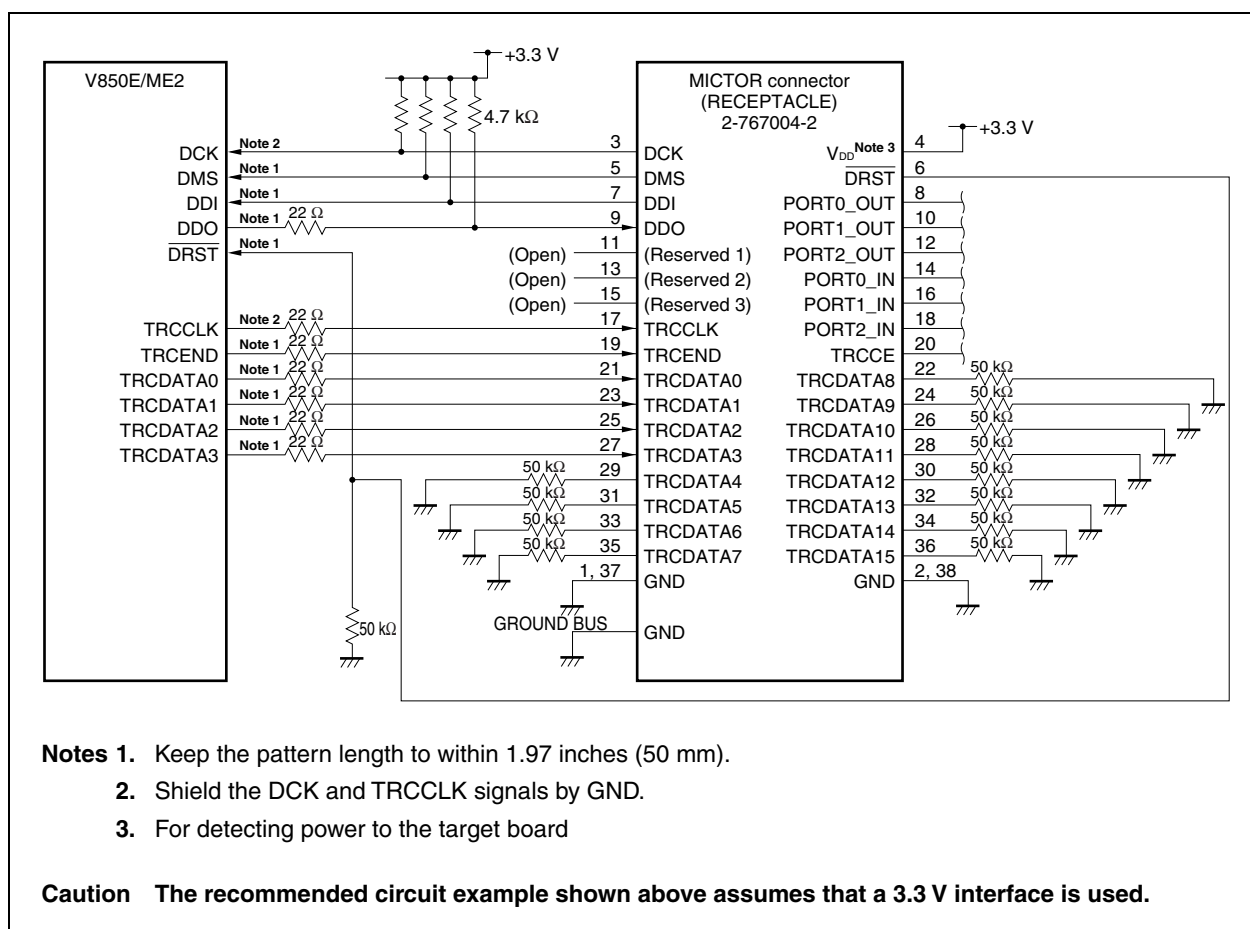
Figure 16-2. Example of Recommended Emulator Connection Circuit
