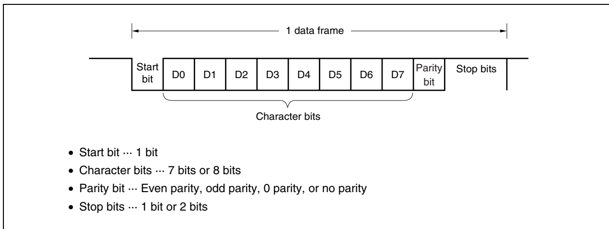
Figure 10-2. Asynchronous Serial Interface Transmit/Receive Data Format (LSB-First Transfer)
