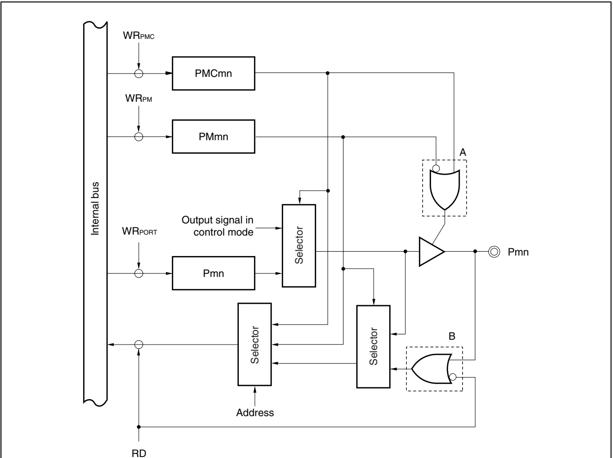
Figure 14-3. Block Diagram of Type D-1
