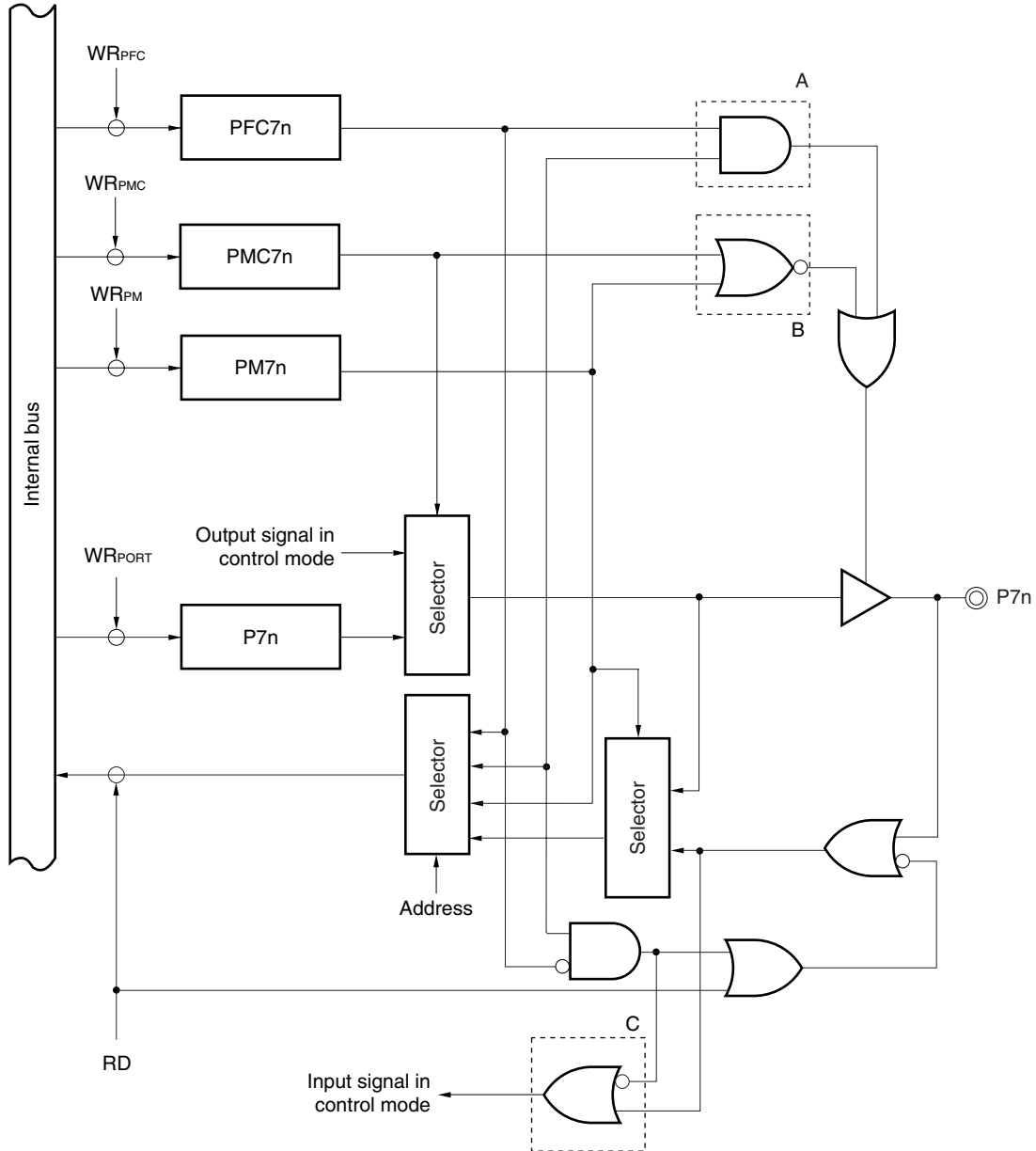
Figure 14-18. Block Diagram of Type L-2
