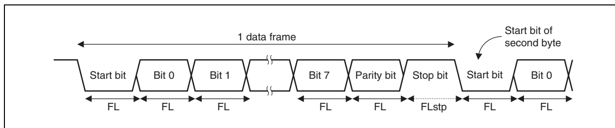
Figure 10-10. Transfer Rate During Continuous Transmission
