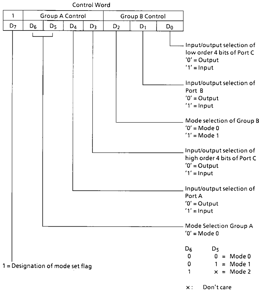
Figure 6.1 Control Word for Mode Selection
