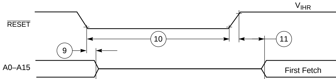
Figure 2-4 Reset Timing
